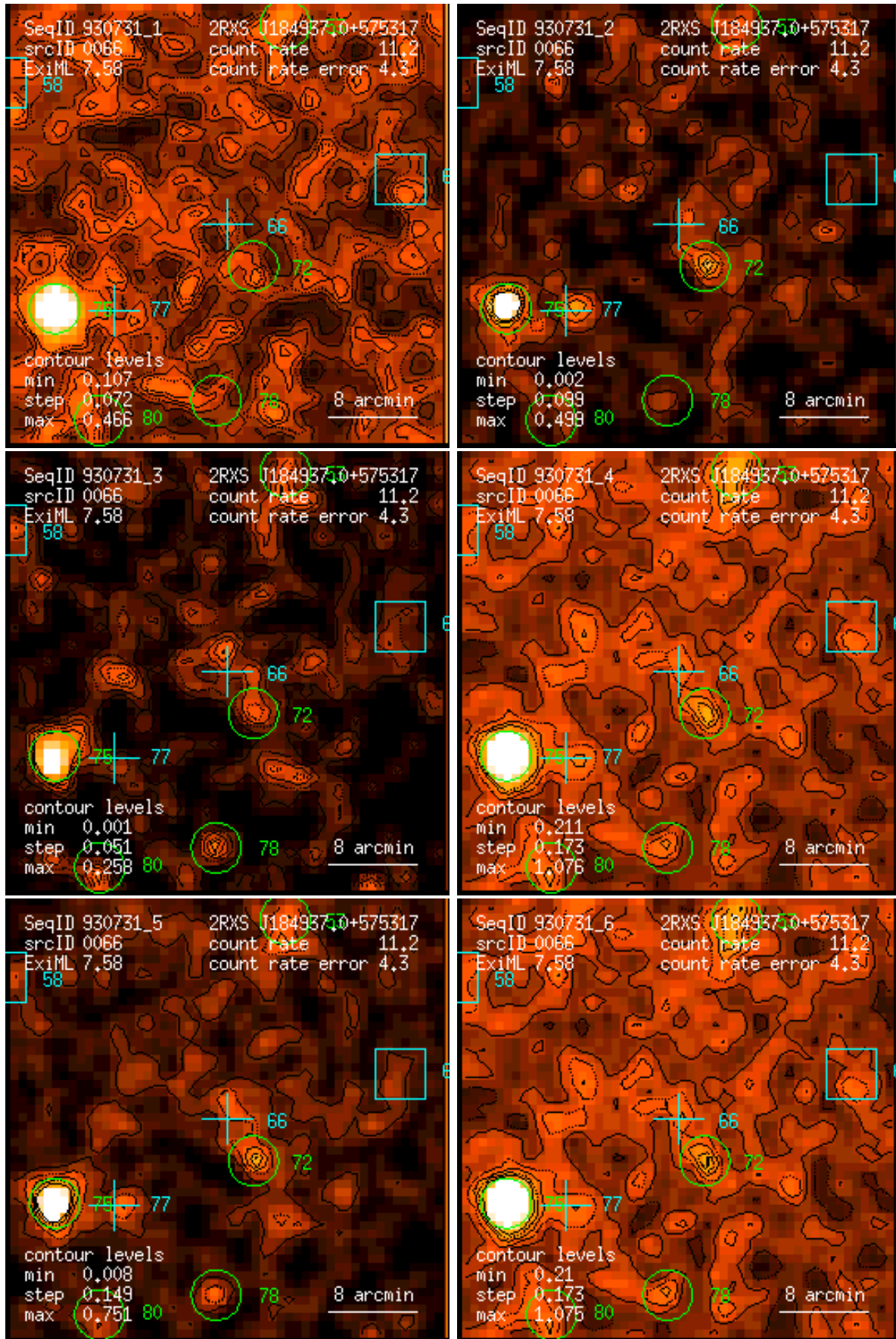
Figure 66: RASS 930731: detection 0066: band rate images, Gaussian filter: (1) PSPC channels 11 – 41, (2) 52 – 90, (3) 91 – 201, (4) 11 – 235, (5) 52 – 201, (6) 11 – 201. Broad band rates in counts/ks. Band rate contour levels in counts/ks/arcmin 2 .
