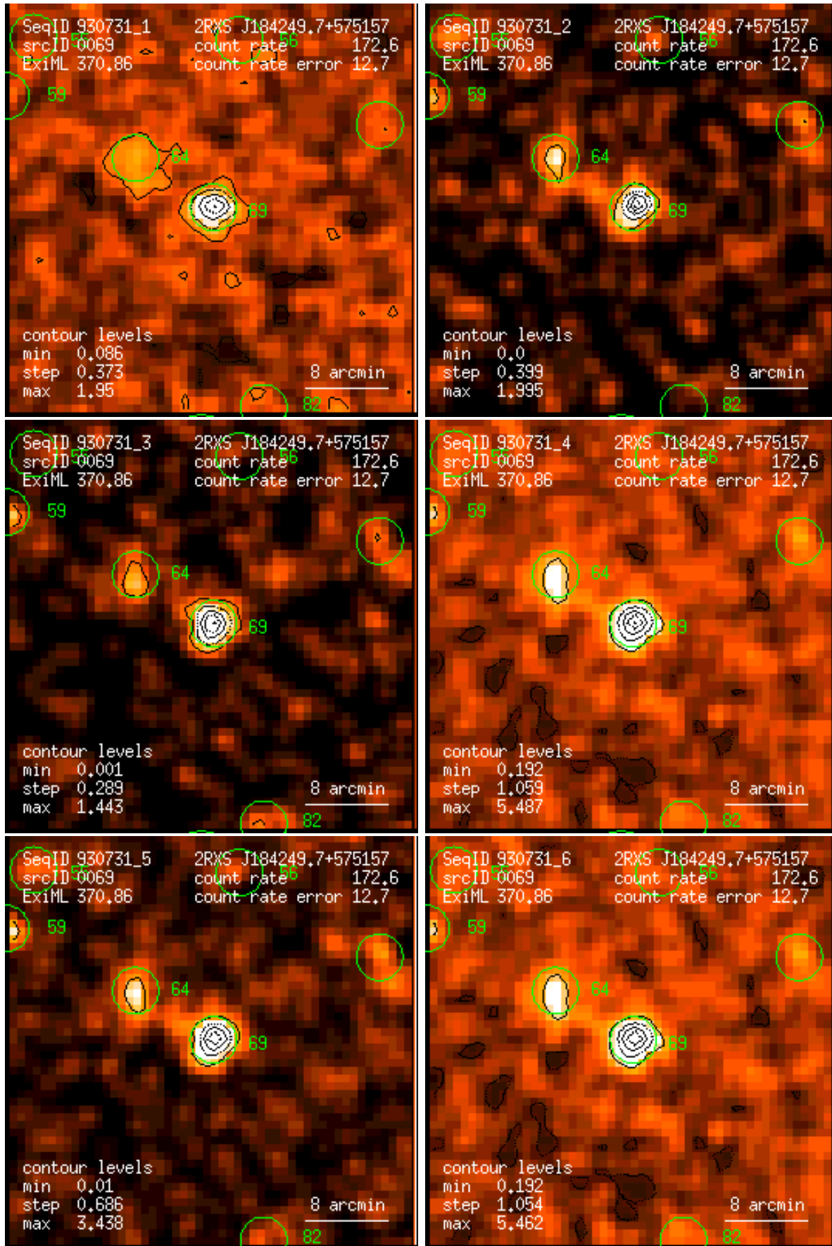
Figure 69: RASS 930731: detection 0069: band rate images, Gaussian filter: (1) PSPC channels 11 – 41, (2) 52 – 90, (3) 91 – 201, (4) 11 – 235, (5) 52 – 201, (6) 11 – 201. Broad band rates in counts/ks. Band rate contour levels in counts/ks/arcmin 2 .
