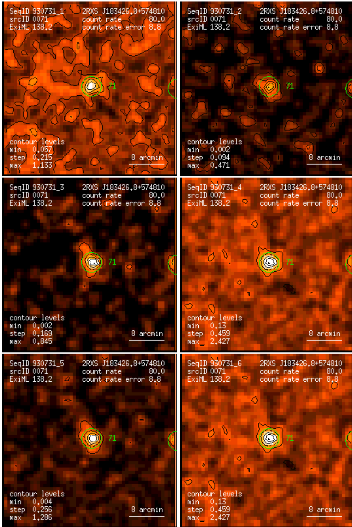
Figure 71: RASS 930731: detection 0071: band rate images, Gaussian filter: (1) PSPC channels 11 – 41, (2) 52 – 90, (3) 91 – 201, (4) 11 – 235, (5) 52 – 201, (6) 11 – 201. Broad band rates in counts/ks. Band rate contour levels in counts/ks/arcmin 2 .
