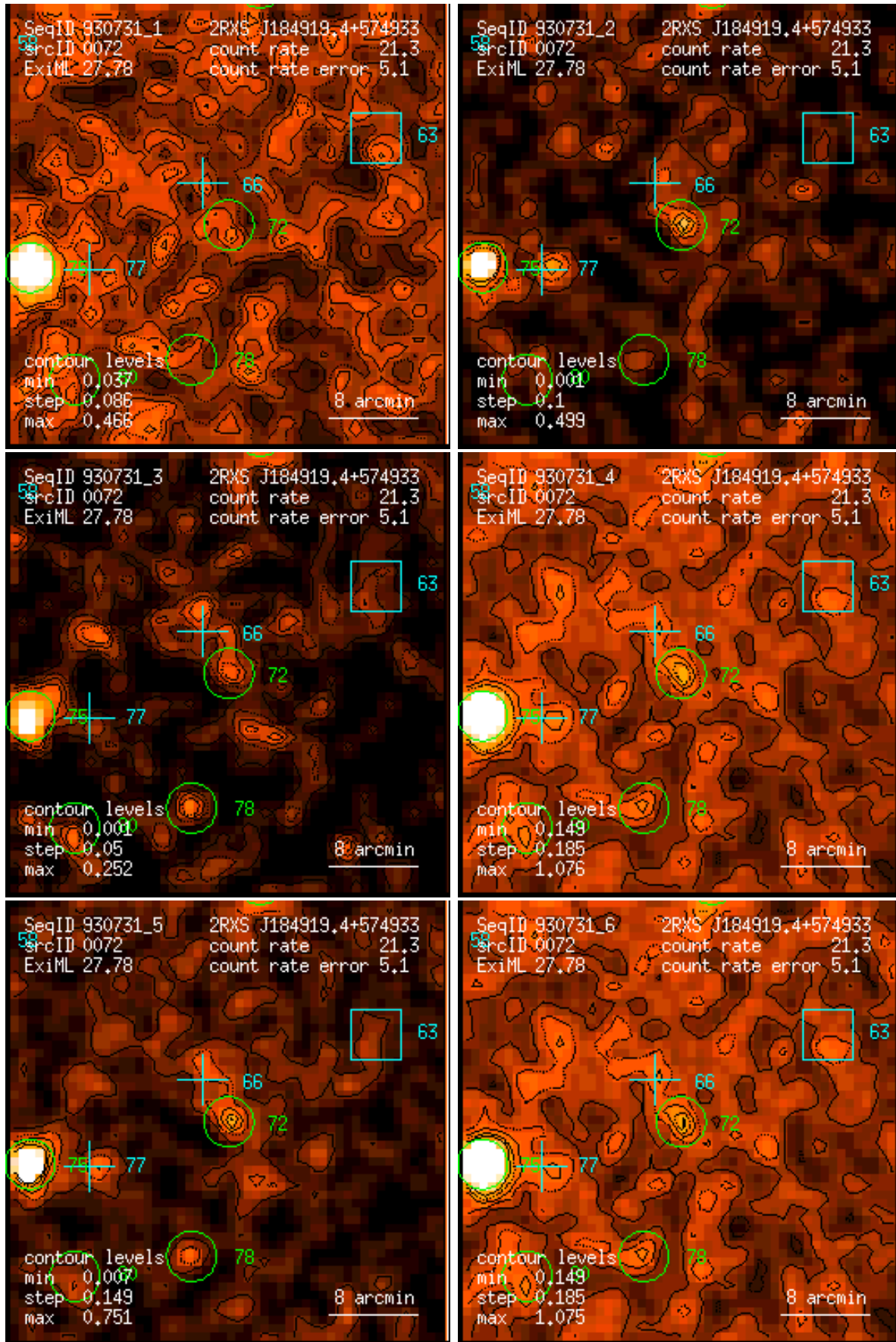
Figure 72: RASS 930731: detection 0072: band rate images, Gaussian filter: (1) PSPC channels 11 – 41, (2) 52 – 90, (3) 91 – 201, (4) 11 – 235, (5) 52 – 201, (6) 11 – 201. Broad band rates in counts/ks. Band rate contour levels in counts/ks/arcmin 2 .
