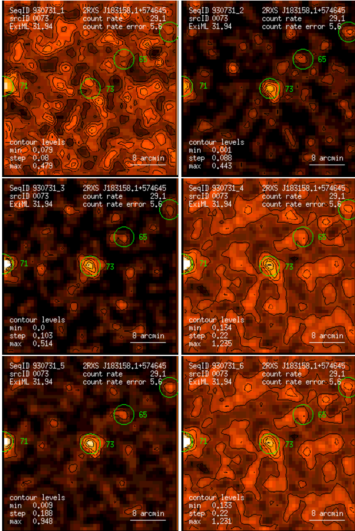
Figure 73: RASS 930731: detection 0073: band rate images, Gaussian filter: (1) PSPC channels 11 – 41, (2) 52 – 90, (3) 91 – 201, (4) 11 – 235, (5) 52 – 201, (6) 11 – 201. Broad band rates in counts/ks. Band rate contour levels in counts/ks/arcmin 2 .
