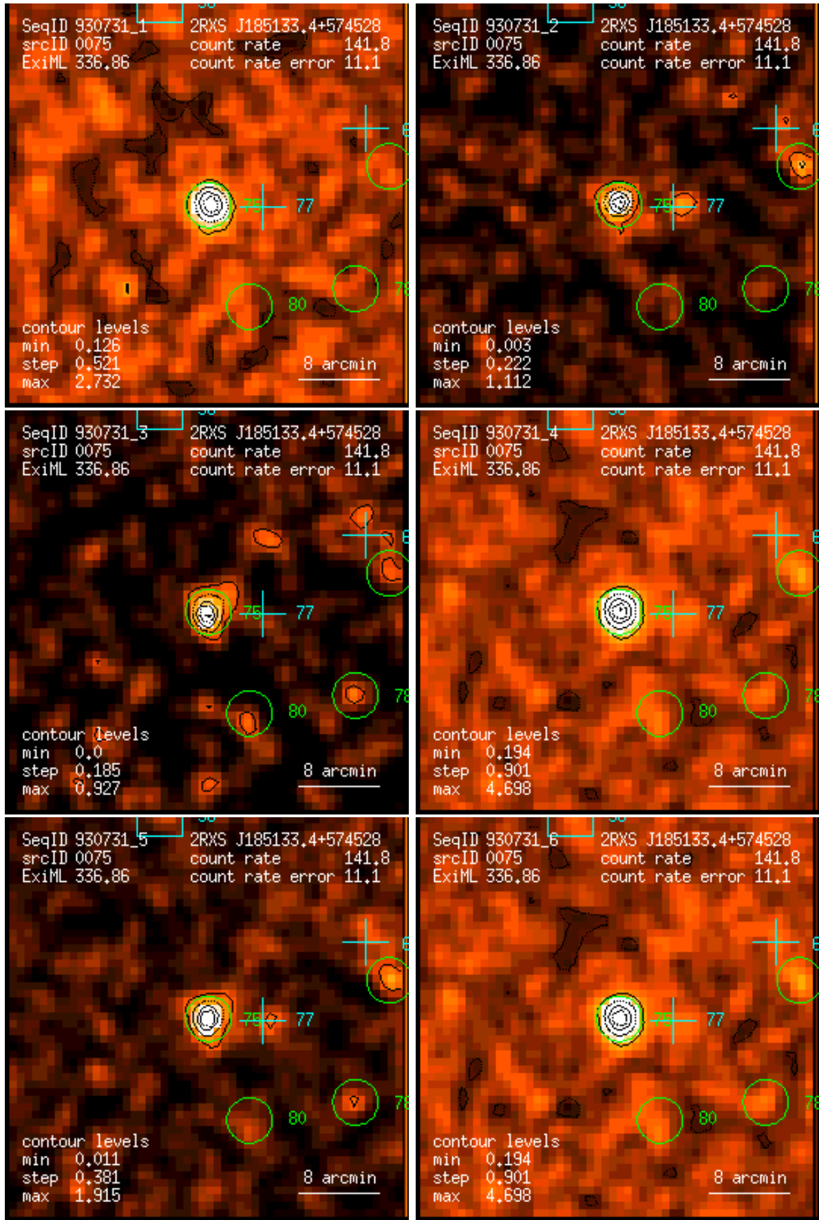
Figure 75: RASS 930731: detection 0075: band rate images, Gaussian filter: (1) PSPC channels 11 – 41, (2) 52 – 90, (3) 91 – 201, (4) 11 – 235, (5) 52 – 201, (6) 11 – 201. Broad band rates in counts/ks. Band rate contour levels in counts/ks/arcmin 2 .
