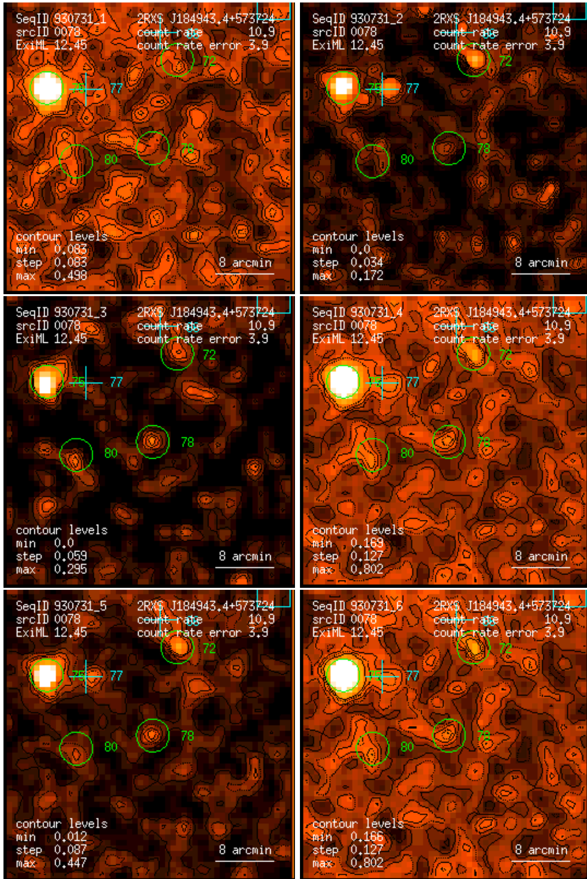
Figure 78: RASS 930731: detection 0078: band rate images, Gaussian filter: (1) PSPC channels 11 – 41, (2) 52 – 90, (3) 91 – 201, (4) 11 – 235, (5) 52 – 201, (6) 11 – 201. Broad band rates in counts/ks. Band rate contour levels in counts/ks/arcmin 2 .
