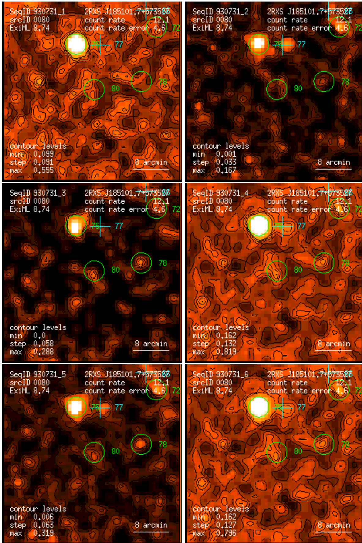
Figure 80: RASS 930731: detection 0080: band rate images, Gaussian filter: (1) PSPC channels 11 – 41, (2) 52 – 90, (3) 91 – 201, (4) 11 – 235, (5) 52 – 201, (6) 11 – 201. Broad band rates in counts/ks. Band rate contour levels in counts/ks/arcmin 2 .
