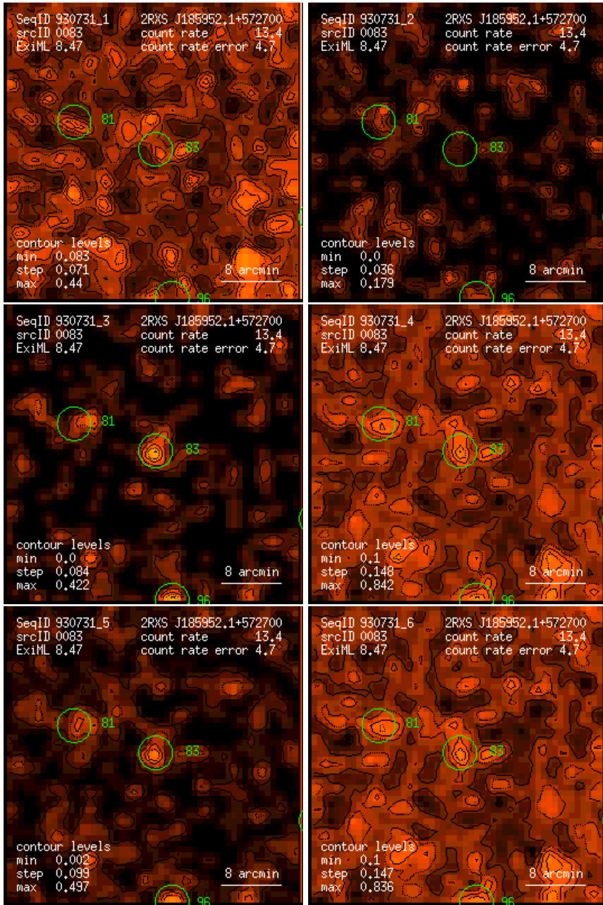
Figure 83: RASS 930731: detection 0083: band rate images, Gaussian filter: (1) PSPC channels 11 – 41, (2) 52 – 90, (3) 91 – 201, (4) 11 – 235, (5) 52 – 201, (6) 11 – 201. Broad band rates in counts/ks. Band rate contour levels in counts/ks/arcmin 2 .
