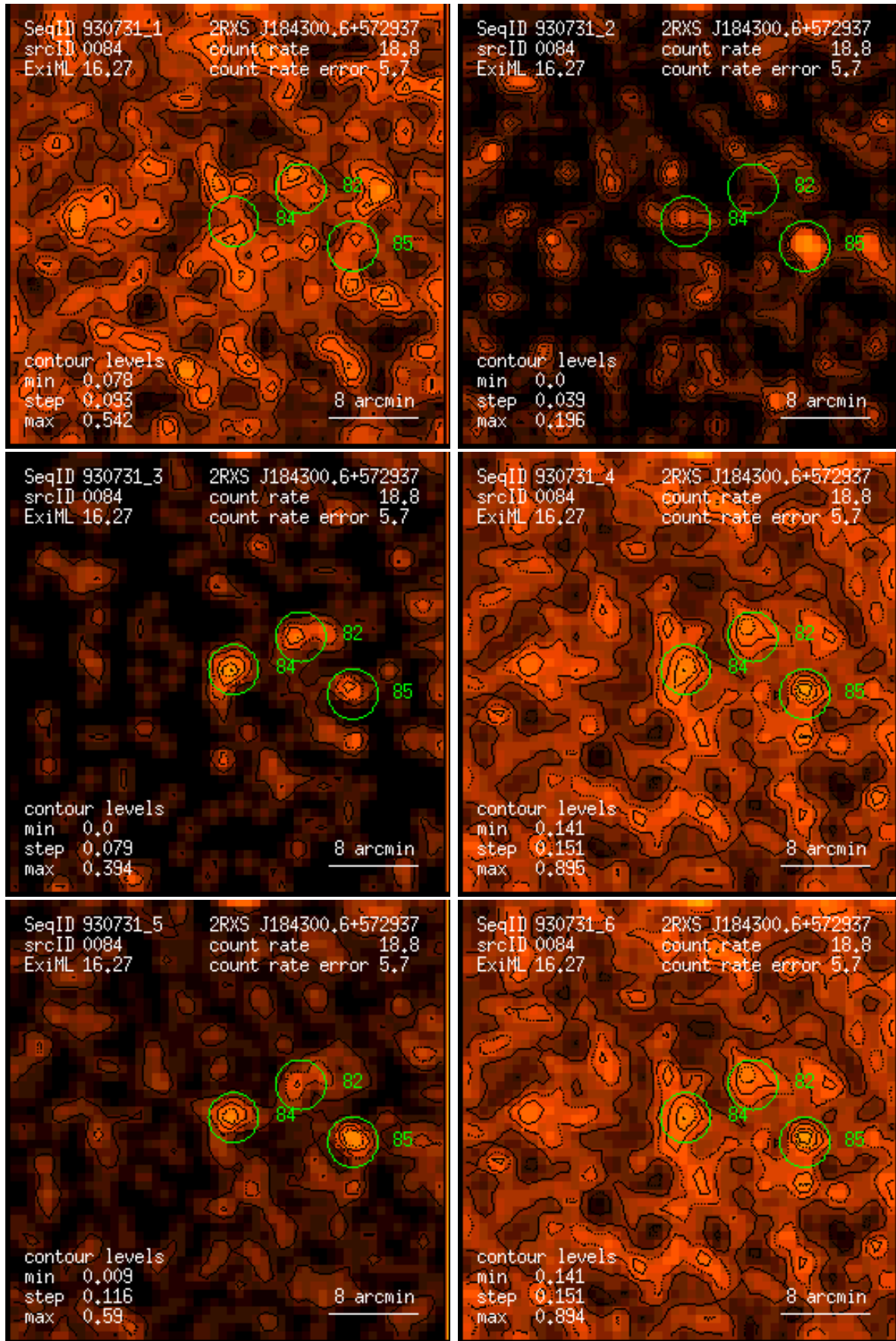
Figure 84: RASS 930731: detection 0084: band rate images, Gaussian filter: (1) PSPC channels 11 – 41, (2) 52 – 90, (3) 91 – 201, (4) 11 – 235, (5) 52 – 201, (6) 11 – 201. Broad band rates in counts/ks. Band rate contour levels in counts/ks/arcmin 2 .
