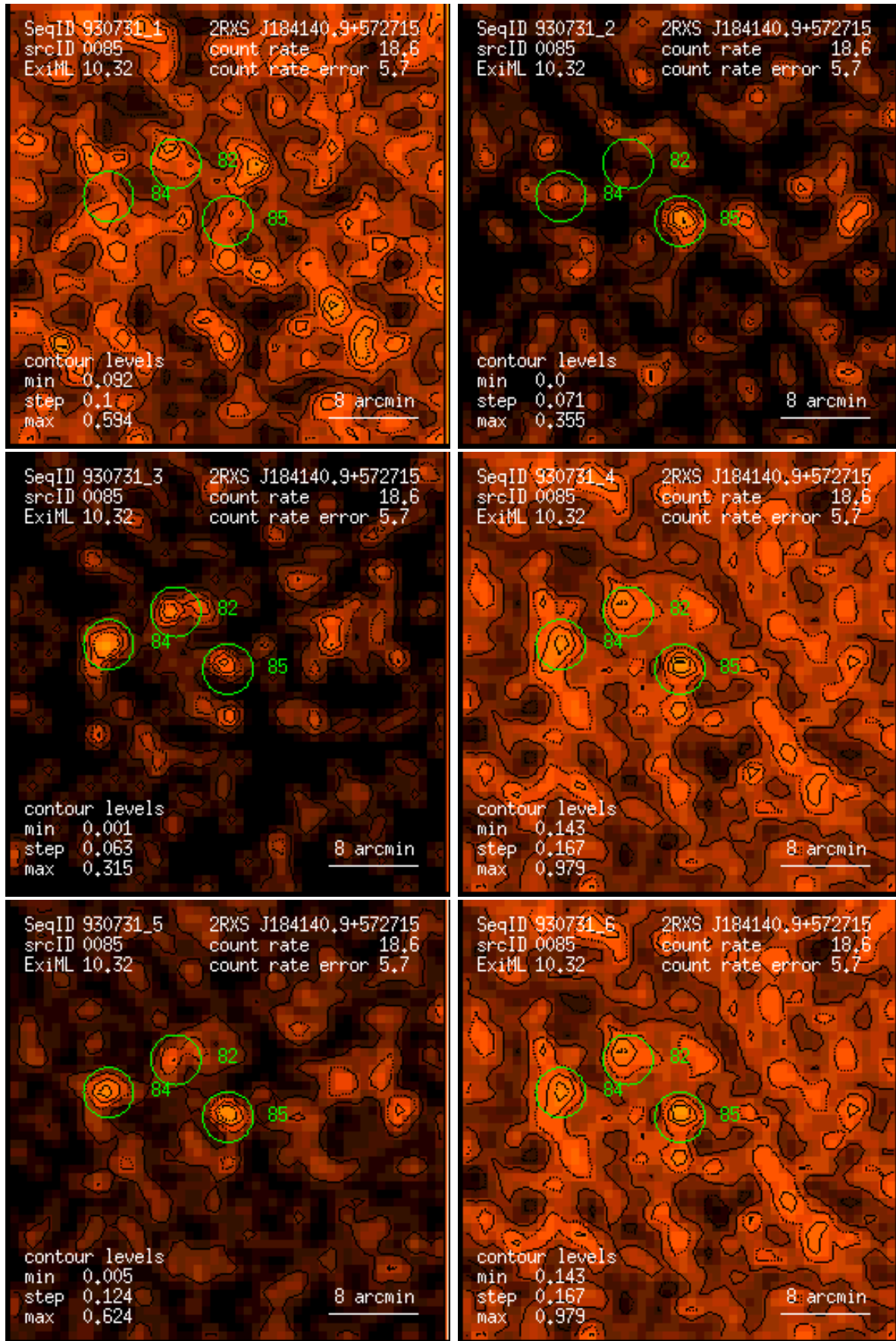
Figure 85: RASS 930731: detection 0085: band rate images, Gaussian filter: (1) PSPC channels 11 – 41, (2) 52 – 90, (3) 91 – 201, (4) 11 – 235, (5) 52 – 201, (6) 11 – 201. Broad band rates in counts/ks. Band rate contour levels in counts/ks/arcmin 2 .
