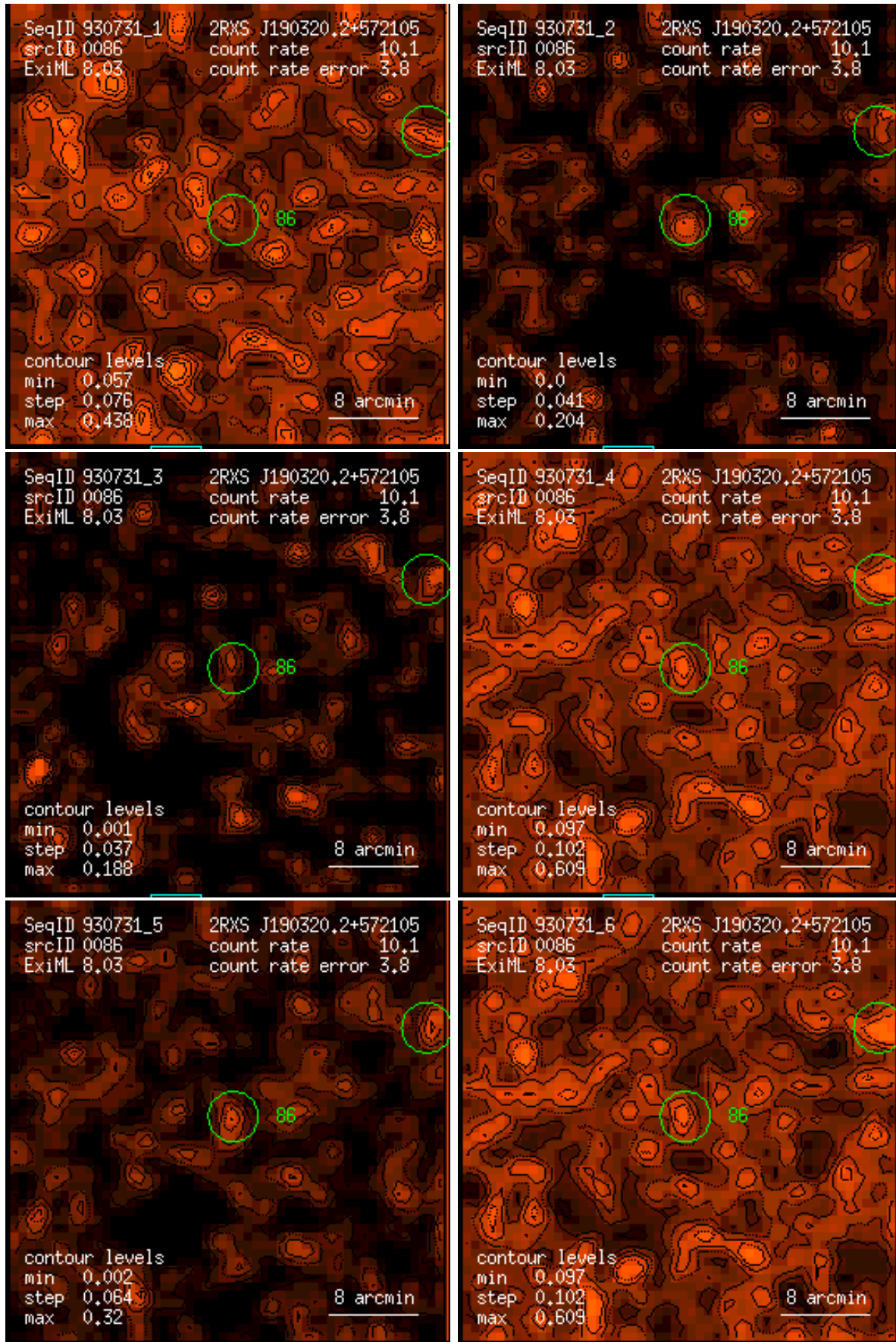
Figure 86: RASS 930731: detection 0086: band rate images, Gaussian filter: (1) PSPC channels 11 – 41, (2) 52 – 90, (3) 91 – 201, (4) 11 – 235, (5) 52 – 201, (6) 11 – 201. Broad band rates in counts/ks. Band rate contour levels in counts/ks/arcmin 2 .
