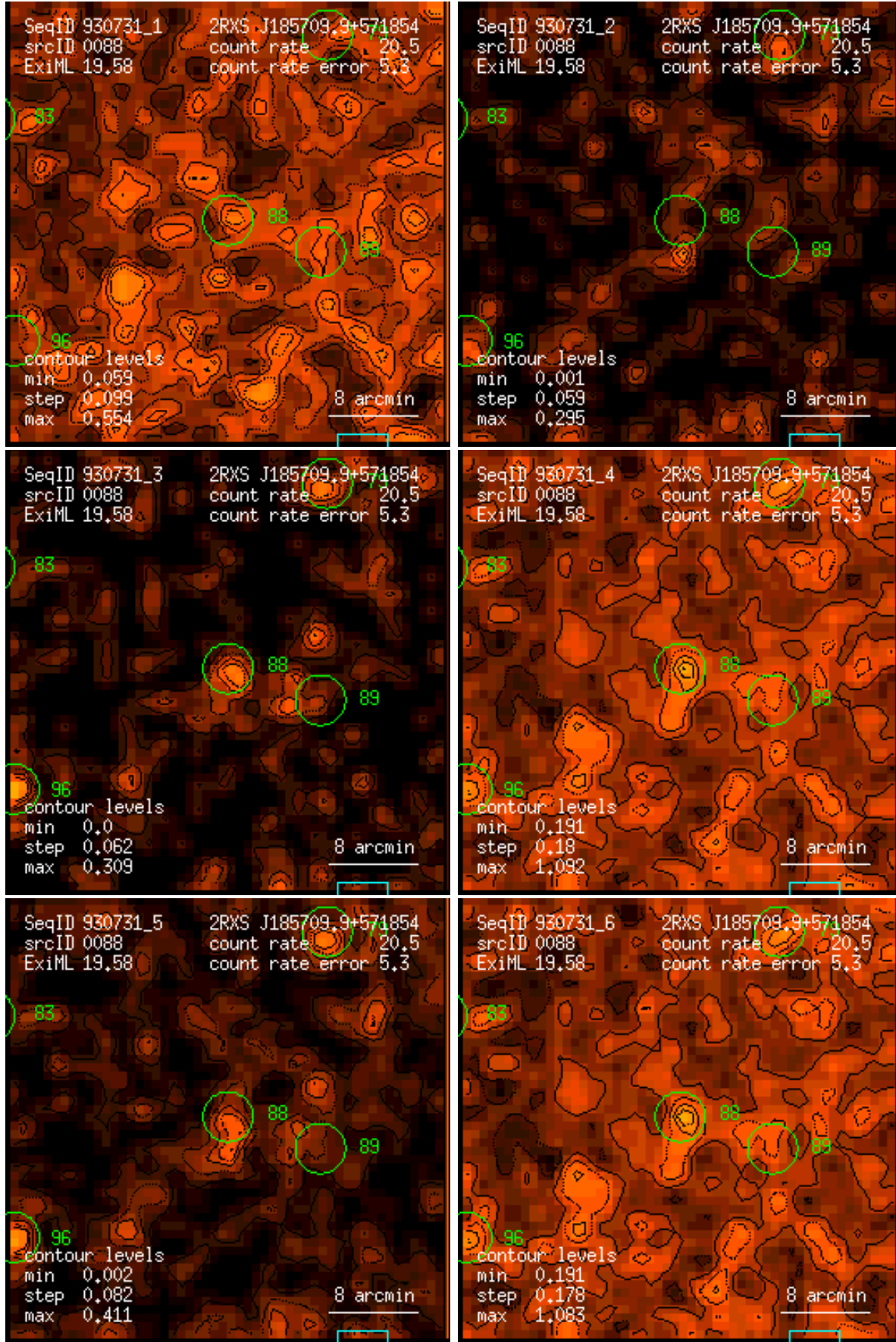
Figure 88: RASS 930731: detection 0088: band rate images, Gaussian filter: (1) PSPC channels 11 – 41, (2) 52 – 90, (3) 91 – 201, (4) 11 – 235, (5) 52 – 201, (6) 11 – 201. Broad band rates in counts/ks. Band rate contour levels in counts/ks/arcmin 2 .
