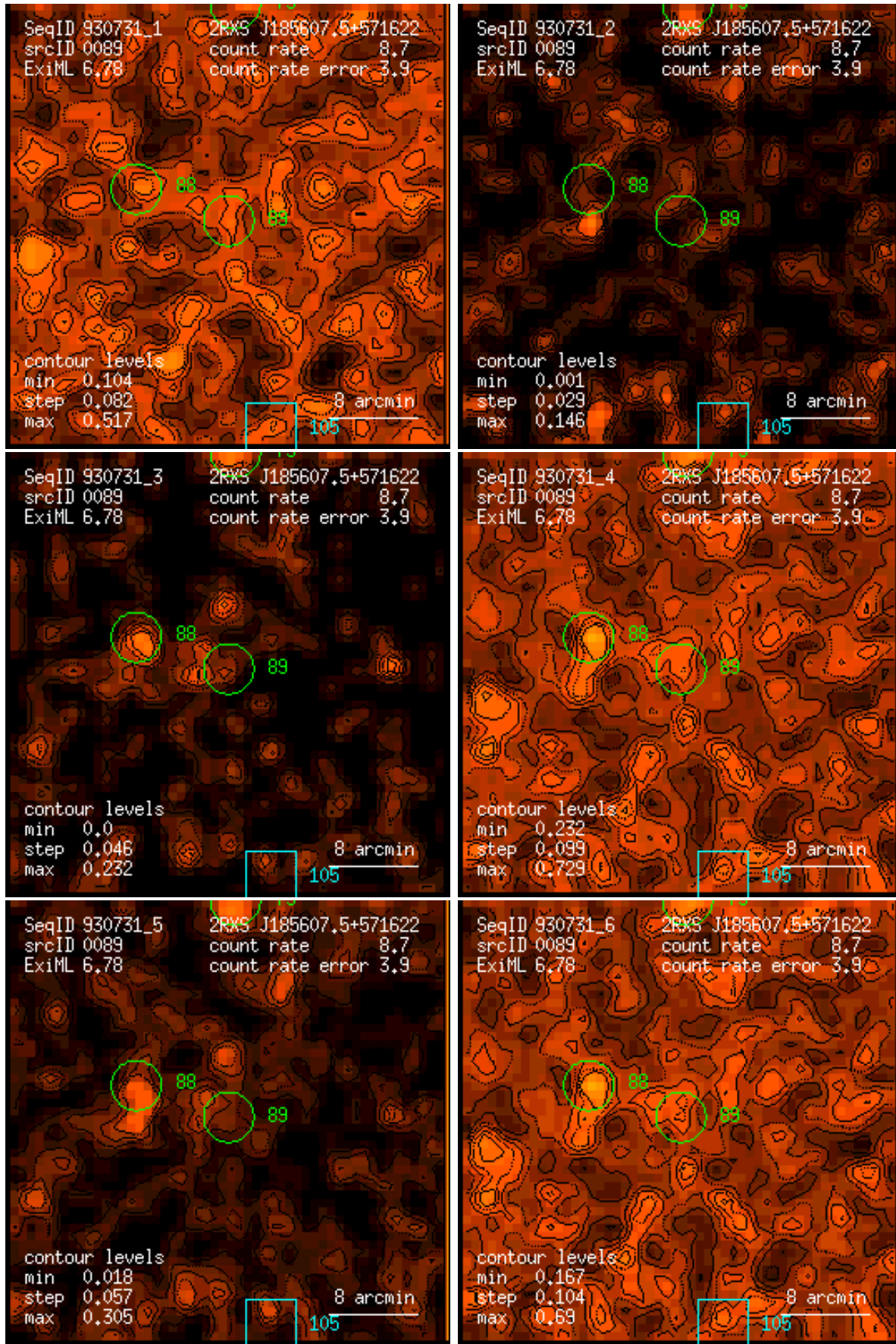
Figure 89: RASS 930731: detection 0089: band rate images, Gaussian filter: (1) PSPC channels 11 – 41, (2) 52 – 90, (3) 91 – 201, (4) 11 – 235, (5) 52 – 201, (6) 11 – 201. Broad band rates in counts/ks. Band rate contour levels in counts/ks/arcmin 2 .
