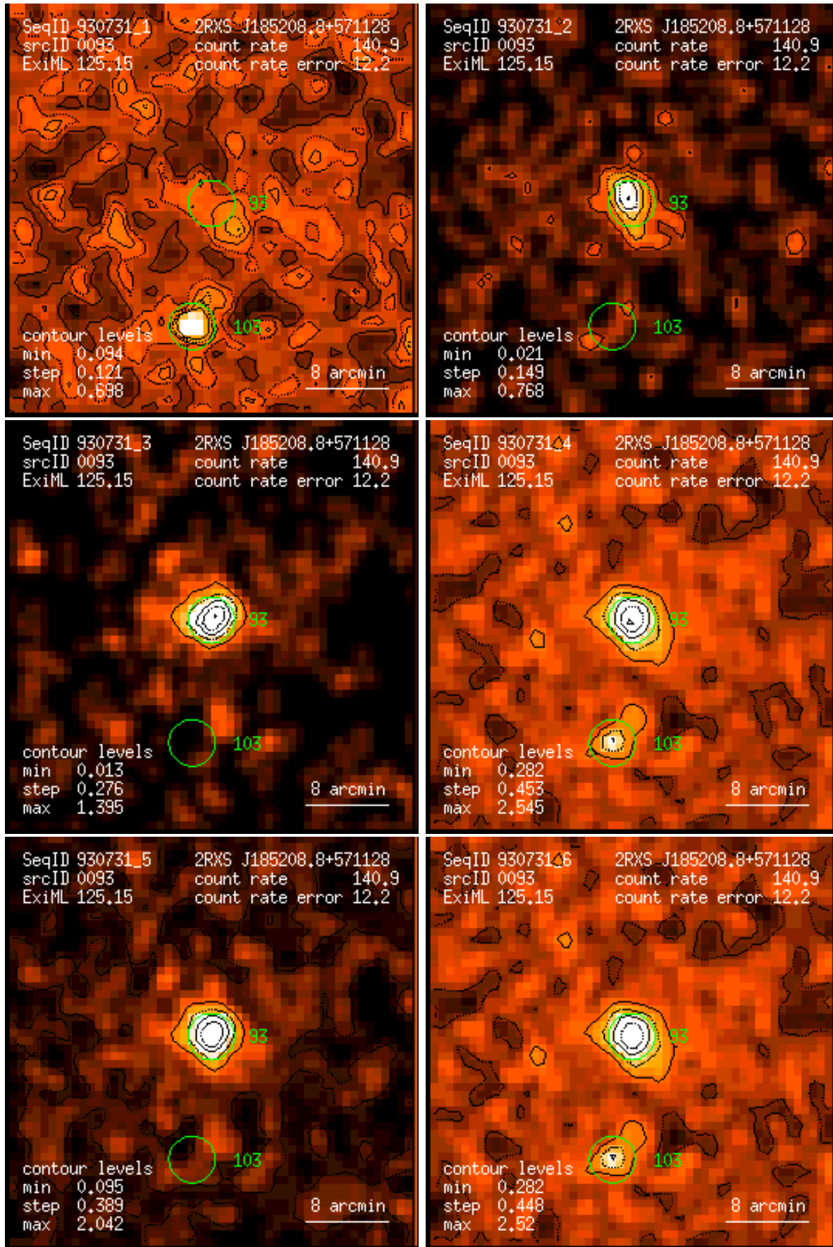
Figure 93: RASS 930731: detection 0093: band rate images, Gaussian filter: (1) PSPC channels 11 – 41, (2) 52 – 90, (3) 91 – 201, (4) 11 – 235, (5) 52 – 201, (6) 11 – 201. Broad band rates in counts/ks. Band rate contour levels in counts/ks/arcmin 2 .
