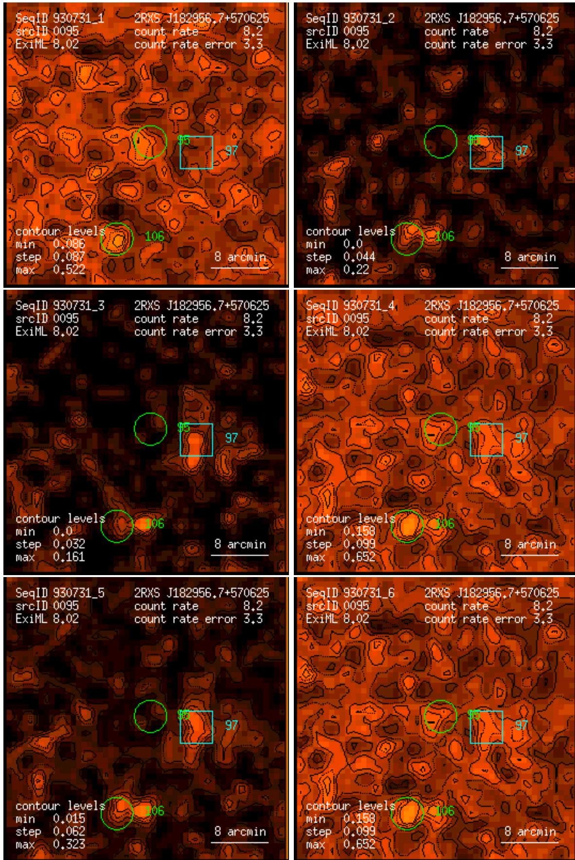
Figure 95: RASS 930731: detection 0095: band rate images, Gaussian filter: (1) PSPC channels 11 – 41, (2) 52 – 90, (3) 91 – 201, (4) 11 – 235, (5) 52 – 201, (6) 11 – 201. Broad band rates in counts/ks. Band rate contour levels in counts/ks/arcmin 2 .
