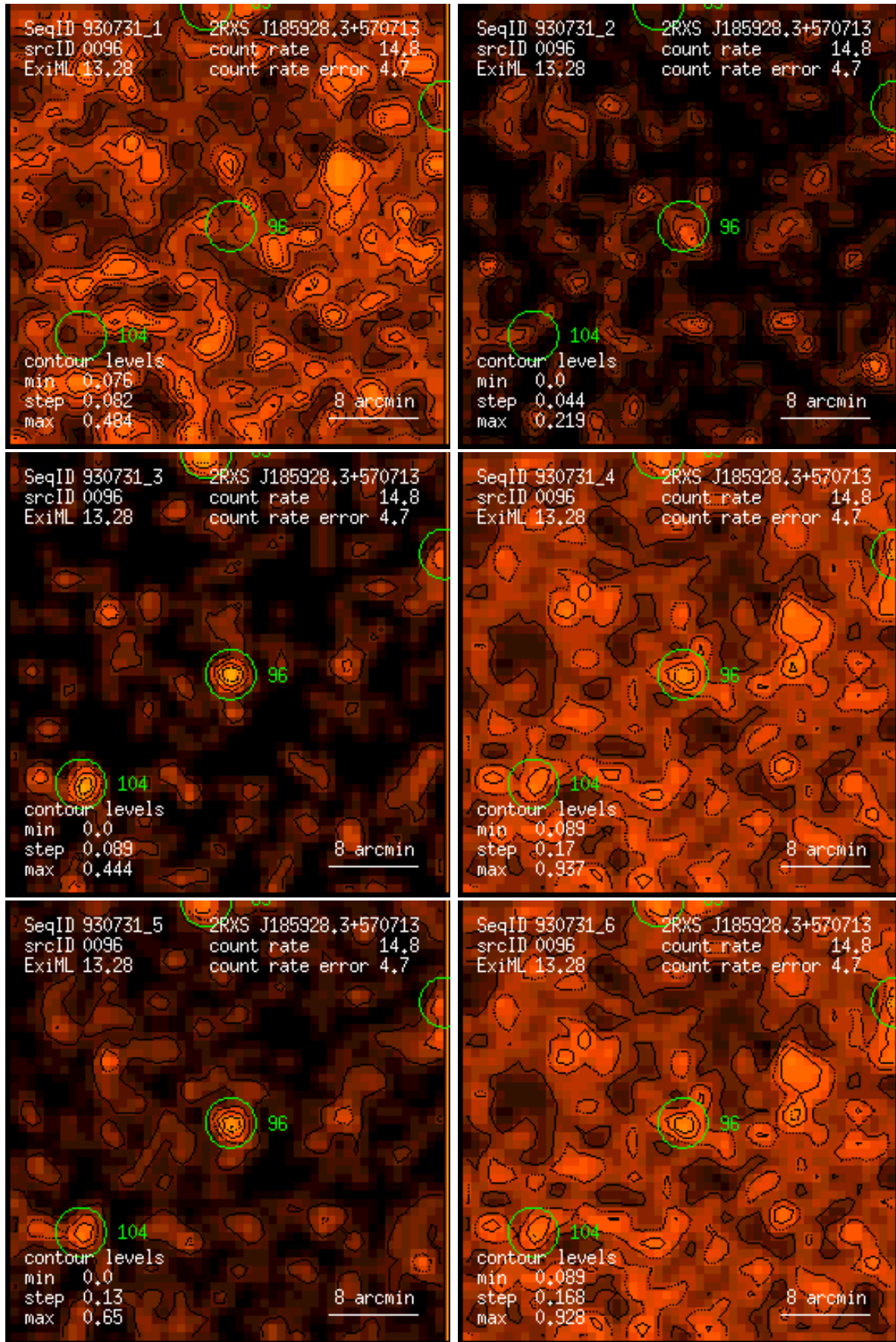
Figure 96: RASS 930731: detection 0096: band rate images, Gaussian filter: (1) PSPC channels 11 – 41, (2) 52 – 90, (3) 91 – 201, (4) 11 – 235, (5) 52 – 201, (6) 11 – 201. Broad band rates in counts/ks. Band rate contour levels in counts/ks/arcmin 2 .
