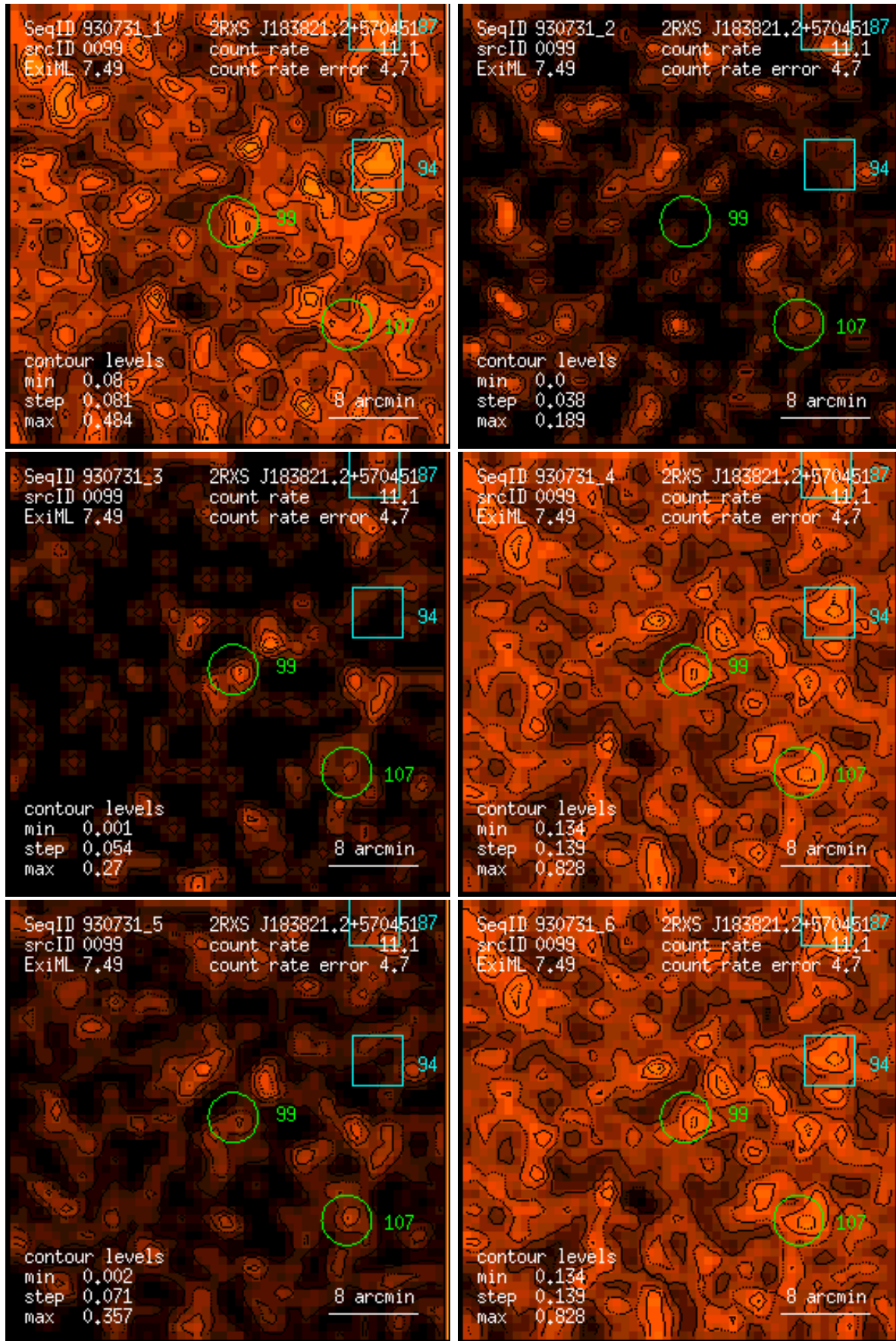
Figure 99: RASS 930731: detection 0099: band rate images, Gaussian filter: (1) PSPC channels 11 – 41, (2) 52 – 90, (3) 91 – 201, (4) 11 – 235, (5) 52 – 201, (6) 11 – 201. Broad band rates in counts/ks. Band rate contour levels in counts/ks/arcmin 2 .
