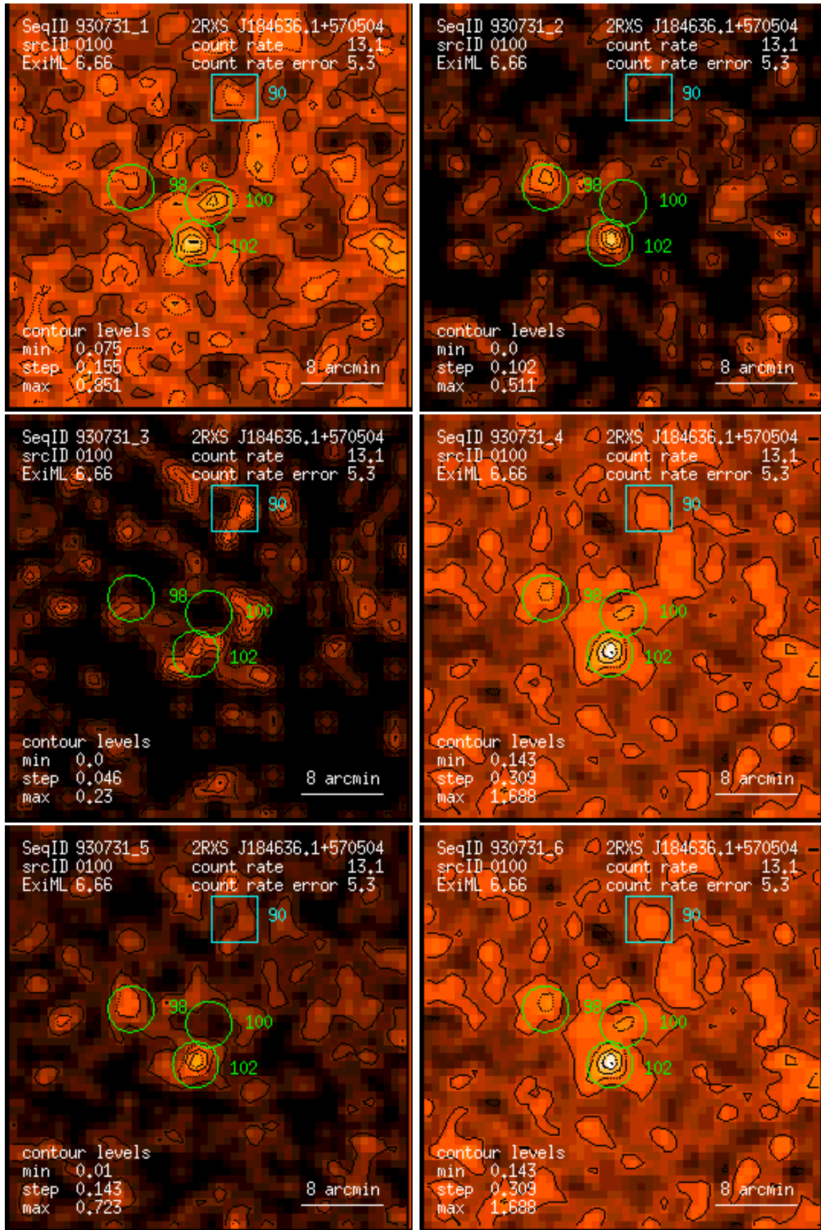
Figure 100: RASS 930731: detection 0100: band rate images, Gaussian filter: (1) PSPC channels 11 – 41, (2) 52 – 90, (3) 91 – 201, (4) 11 – 235, (5) 52 – 201, (6) 11 – 201. Broad band rates in counts/ks. Band rate contour levels in counts/ks/arcmin 2 .
