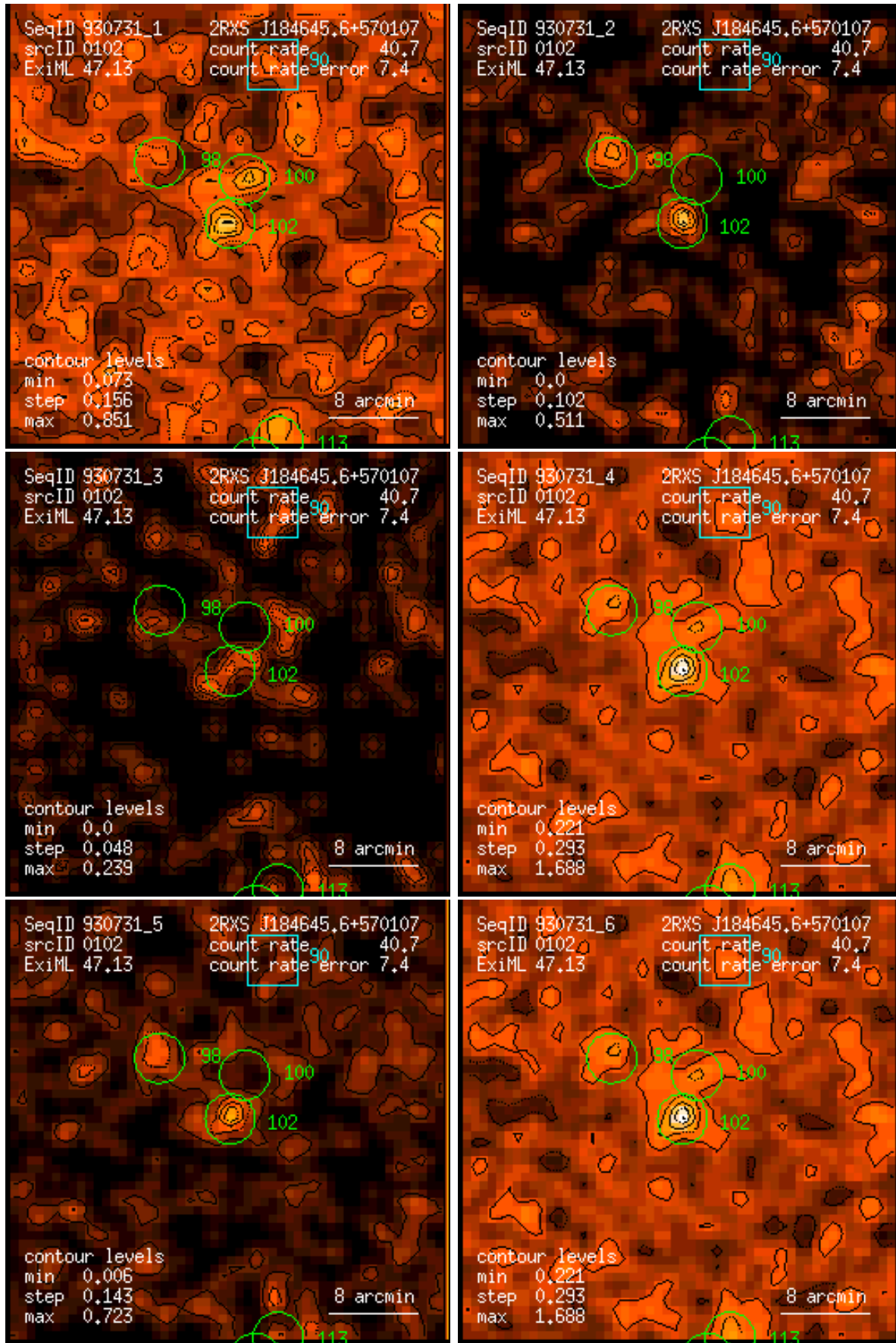
Figure 102: RASS 930731: detection 0102: band rate images, Gaussian filter: (1) PSPC channels 11 – 41, (2) 52 – 90, (3) 91 – 201, (4) 11 – 235, (5) 52 – 201, (6) 11 – 201. Broad band rates in counts/ks. Band rate contour levels in counts/ks/arcmin 2 .
