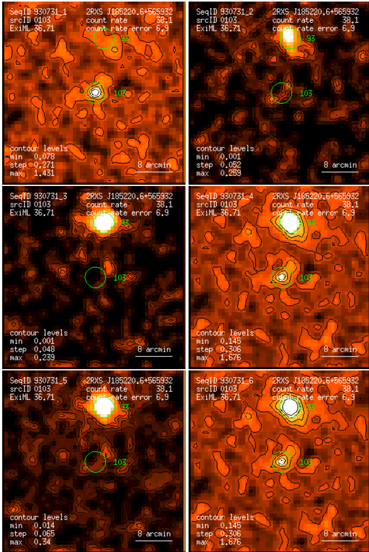
Figure 103: RASS 930731: detection 0103: band rate images, Gaussian filter: (1) PSPC channels 11 – 41, (2) 52 – 90, (3) 91 – 201, (4) 11 – 235, (5) 52 – 201, (6) 11 – 201. Broad band rates in counts/ks. Band rate contour levels in counts/ks/arcmin 2 .
