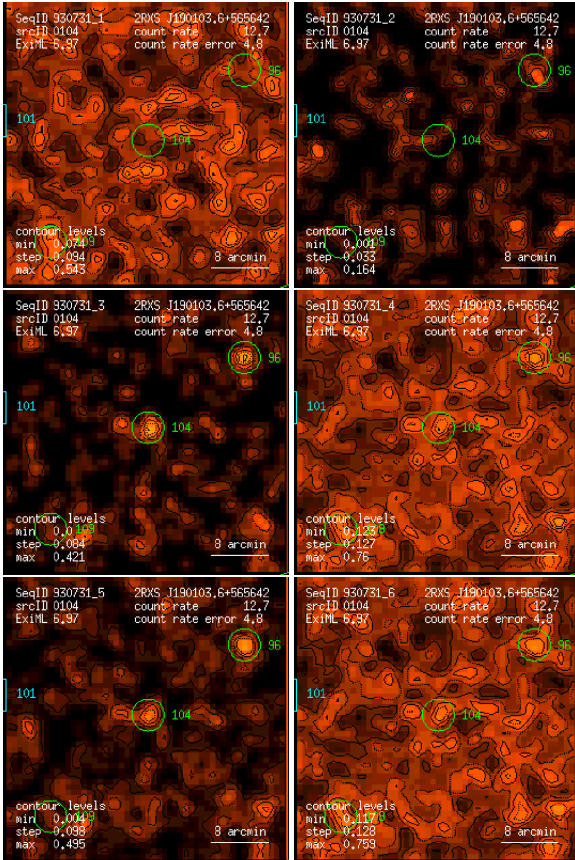
Figure 104: RASS 930731: detection 0104: band rate images, Gaussian filter: (1) PSPC channels 11 – 41, (2) 52 – 90, (3) 91 – 201, (4) 11 – 235, (5) 52 – 201, (6) 11 – 201. Broad band rates in counts/ks. Band rate contour levels in counts/ks/arcmin 2 .
