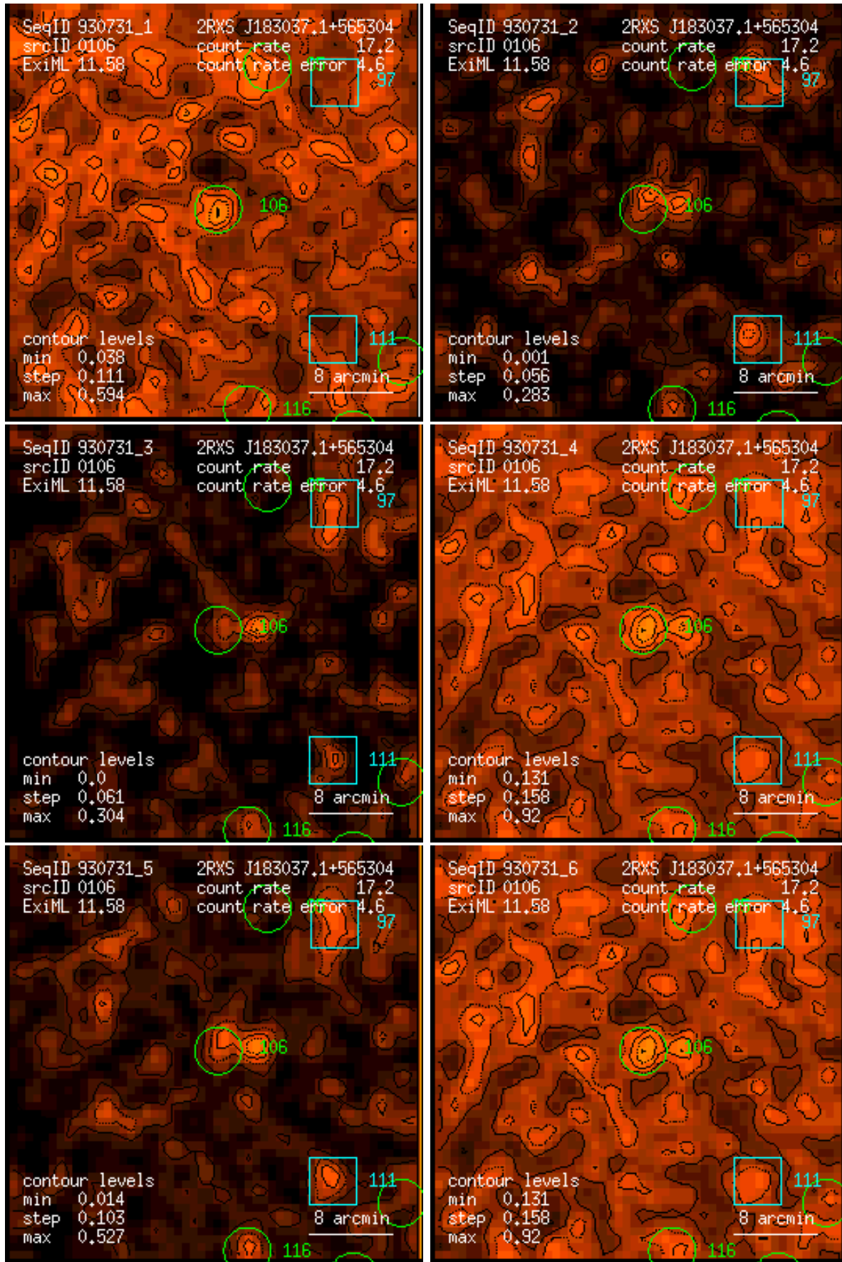
Figure 106: RASS 930731: detection 0106: band rate images, Gaussian filter: (1) PSPC channels 11 – 41, (2) 52 – 90, (3) 91 – 201, (4) 11 – 235, (5) 52 – 201, (6) 11 – 201. Broad band rates in counts/ks. Band rate contour levels in counts/ks/arcmin 2 .
