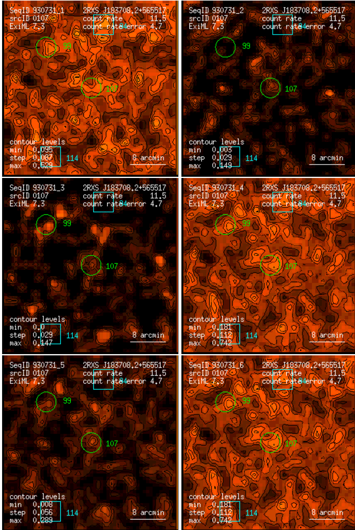
Figure 107: RASS 930731: detection 0107: band rate images, Gaussian filter: (1) PSPC channels 11 – 41, (2) 52 – 90, (3) 91 – 201, (4) 11 – 235, (5) 52 – 201, (6) 11 – 201. Broad band rates in counts/ks. Band rate contour levels in counts/ks/arcmin 2 .
