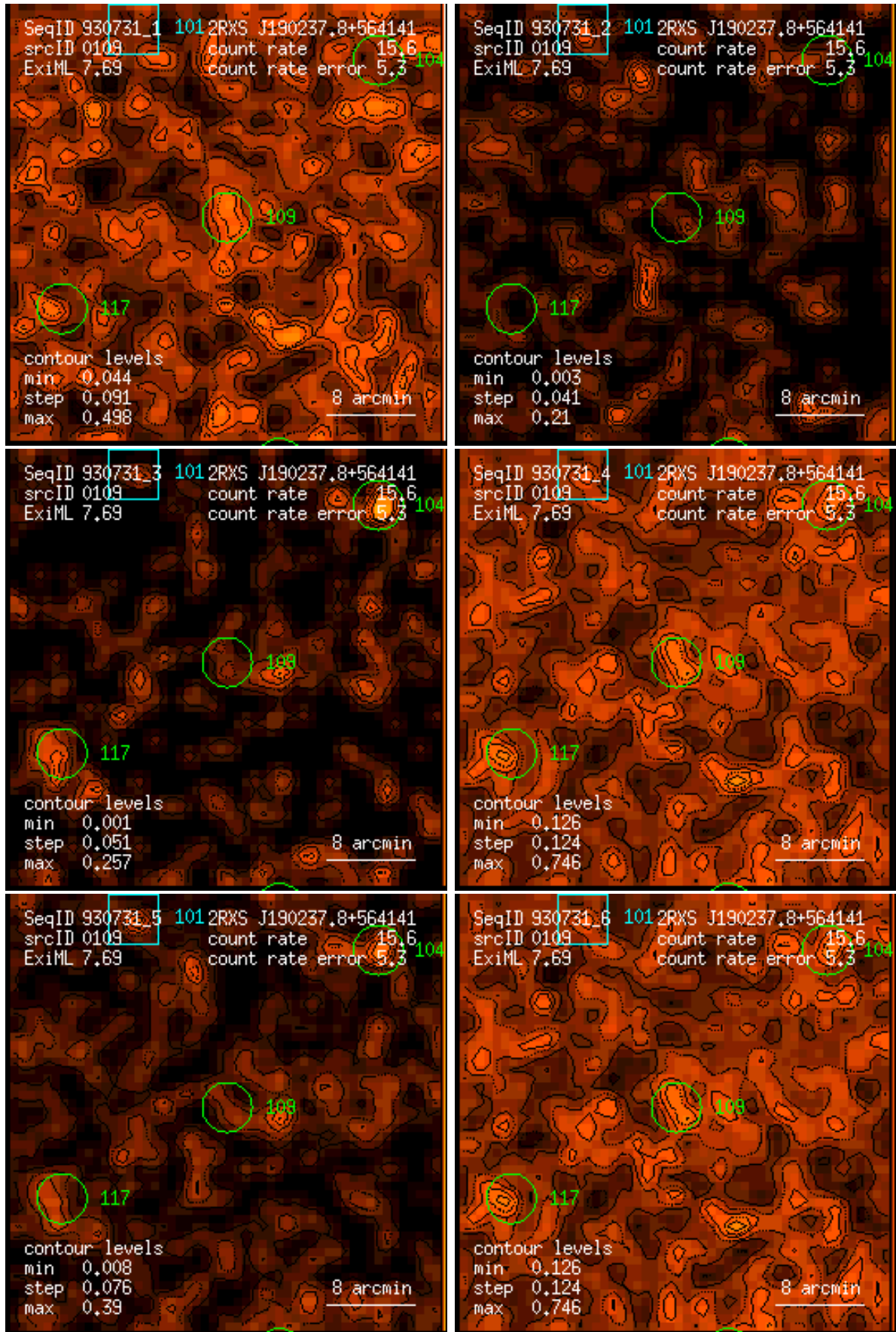
Figure 109: RASS 930731: detection 0109: band rate images, Gaussian filter: (1) PSPC channels 11 – 41, (2) 52 – 90, (3) 91 – 201, (4) 11 – 235, (5) 52 – 201, (6) 11 – 201. Broad band rates in counts/ks. Band rate contour levels in counts/ks/arcmin 2 .
