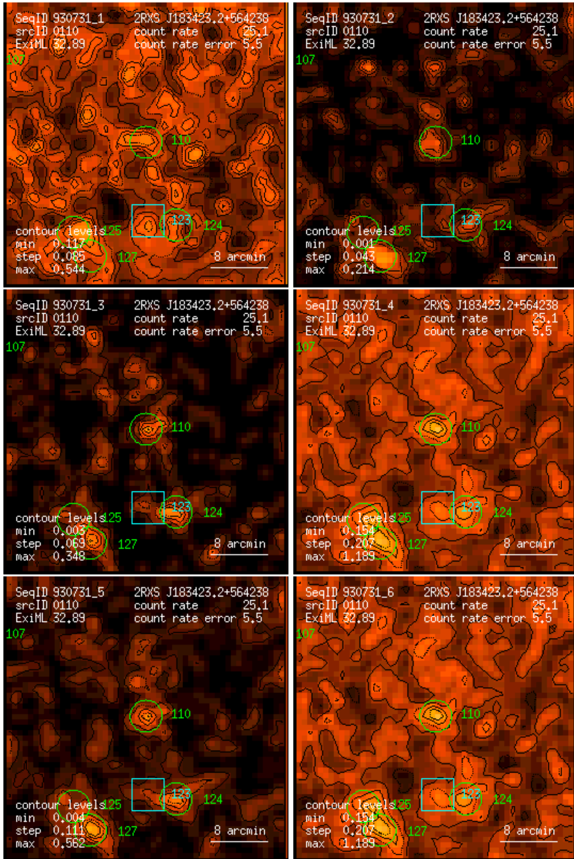
Figure 110: RASS 930731: detection 0110: band rate images, Gaussian filter: (1) PSPC channels 11 – 41, (2) 52 – 90, (3) 91 – 201, (4) 11 – 235, (5) 52 – 201, (6) 11 – 201. Broad band rates in counts/ks. Band rate contour levels in counts/ks/arcmin 2 .
