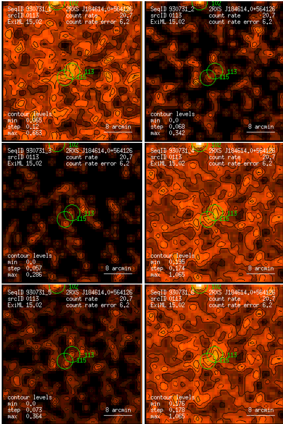
Figure 113: RASS 930731: detection 0113: band rate images, Gaussian filter: (1) PSPC channels 11 – 41, (2) 52 – 90, (3) 91 – 201, (4) 11 – 235, (5) 52 – 201, (6) 11 – 201. Broad band rates in counts/ks. Band rate contour levels in counts/ks/arcmin 2 .
