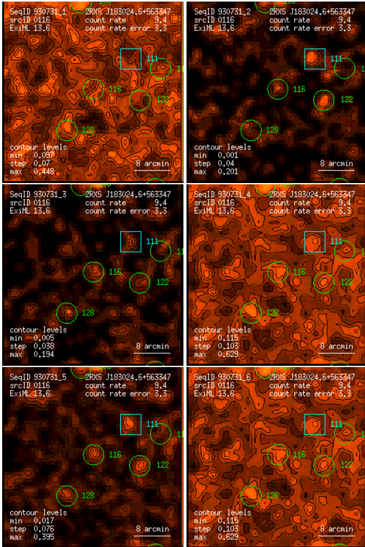
Figure 116: RASS 930731: detection 0116: band rate images, Gaussian filter: (1) PSPC channels 11 – 41, (2) 52 – 90, (3) 91 – 201, (4) 11 – 235, (5) 52 – 201, (6) 11 – 201. Broad band rates in counts/ks. Band rate contour levels in counts/ks/arcmin 2 .
