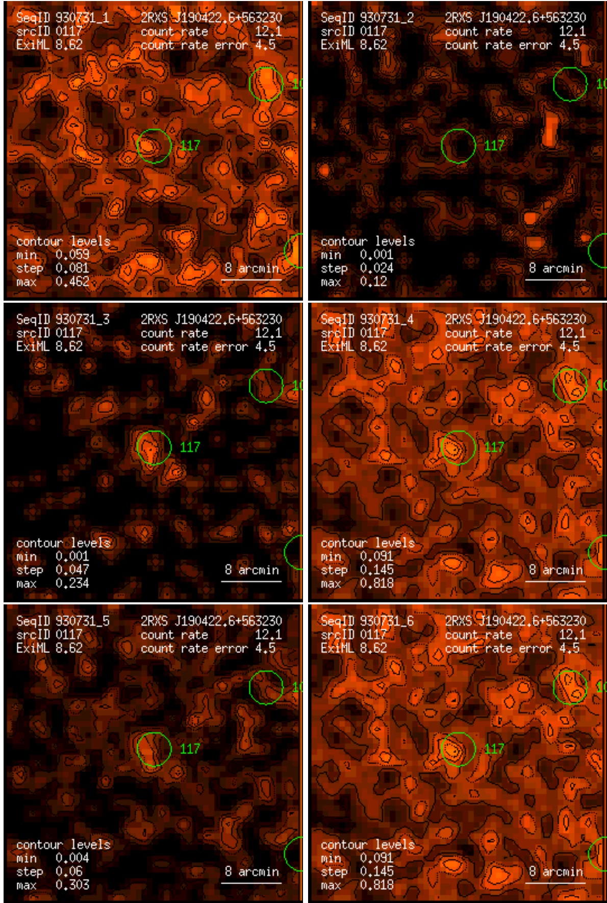
Figure 117: RASS 930731: detection 0117: band rate images, Gaussian filter: (1) PSPC channels 11 – 41, (2) 52 – 90, (3) 91 – 201, (4) 11 – 235, (5) 52 – 201, (6) 11 – 201. Broad band rates in counts/ks. Band rate contour levels in counts/ks/arcmin 2 .
