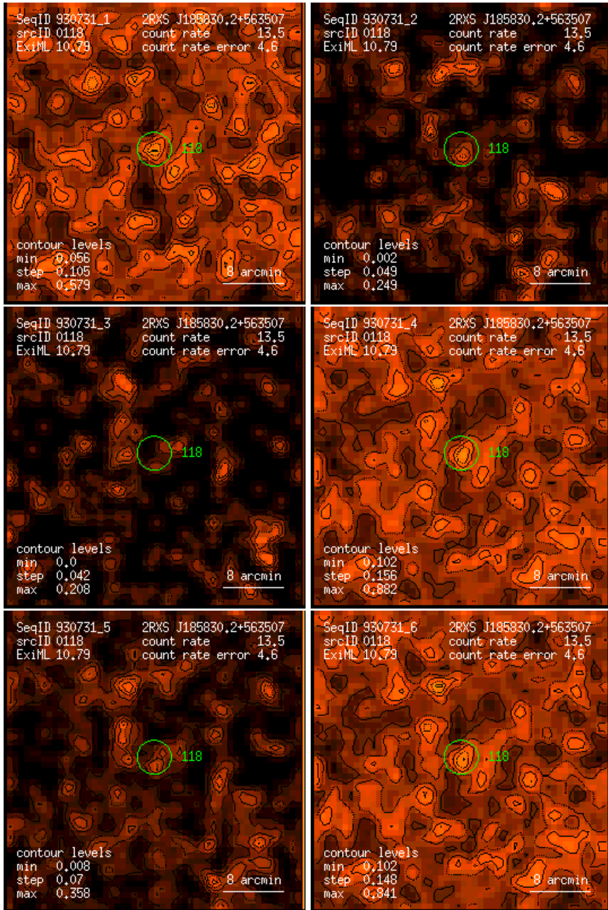
Figure 118: RASS 930731: detection 0118: band rate images, Gaussian filter: (1) PSPC channels 11 – 41, (2) 52 – 90, (3) 91 – 201, (4) 11 – 235, (5) 52 – 201, (6) 11 – 201. Broad band rates in counts/ks. Band rate contour levels in counts/ks/arcmin 2 .
