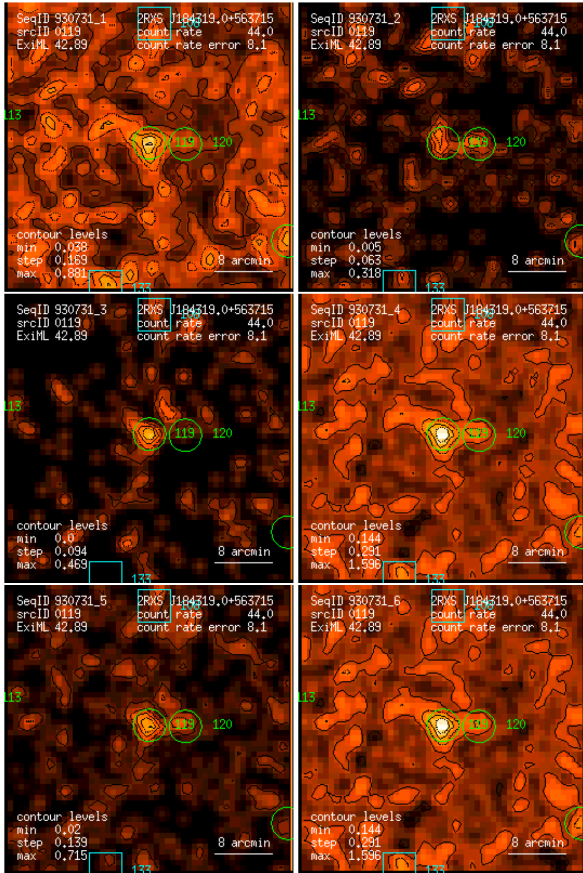
Figure 119: RASS 930731: detection 0119: band rate images, Gaussian filter: (1) PSPC channels 11 – 41, (2) 52 – 90, (3) 91 – 201, (4) 11 – 235, (5) 52 – 201, (6) 11 – 201. Broad band rates in counts/ks. Band rate contour levels in counts/ks/arcmin 2 .
