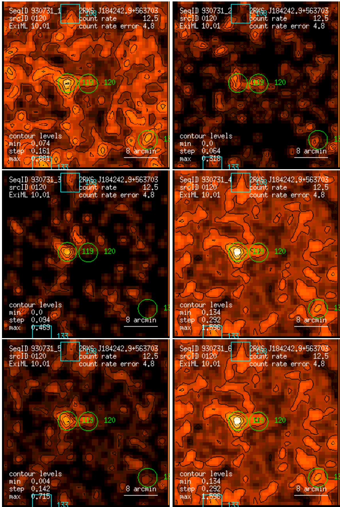
Figure 120: RASS 930731: detection 0120: band rate images, Gaussian filter: (1) PSPC channels 11 – 41, (2) 52 – 90, (3) 91 – 201, (4) 11 – 235, (5) 52 – 201, (6) 11 – 201. Broad band rates in counts/ks. Band rate contour levels in counts/ks/arcmin 2 .
