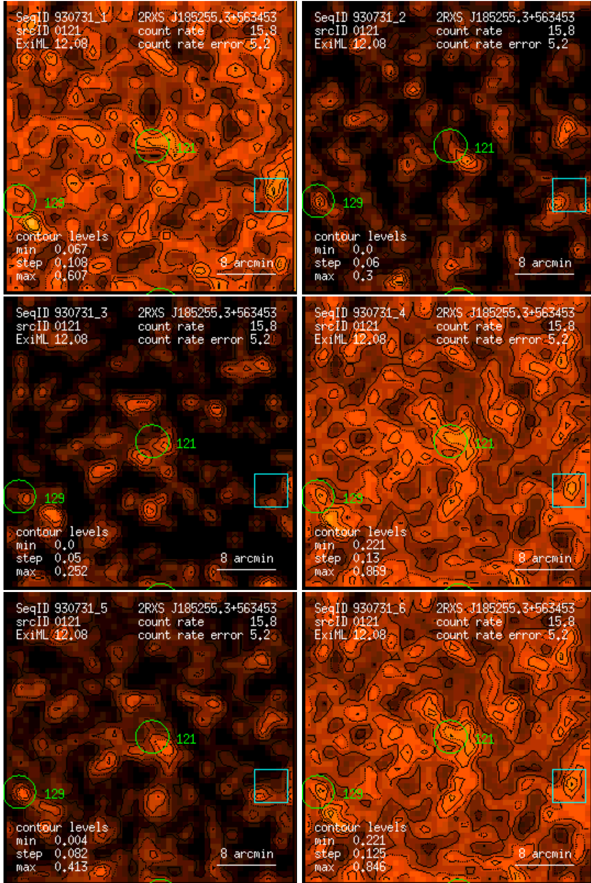
Figure 121: RASS 930731: detection 0121: band rate images, Gaussian filter: (1) PSPC channels 11 – 41, (2) 52 – 90, (3) 91 – 201, (4) 11 – 235, (5) 52 – 201, (6) 11 – 201. Broad band rates in counts/ks. Band rate contour levels in counts/ks/arcmin 2 .
