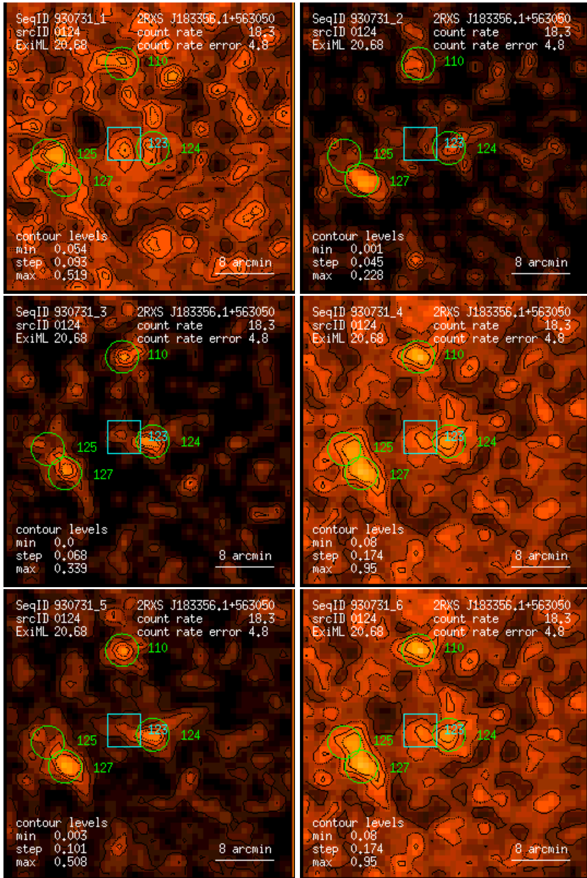
Figure 124: RASS 930731: detection 0124: band rate images, Gaussian filter: (1) PSPC channels 11 – 41, (2) 52 – 90, (3) 91 – 201, (4) 11 – 235, (5) 52 – 201, (6) 11 – 201. Broad band rates in counts/ks. Band rate contour levels in counts/ks/arcmin 2 .
