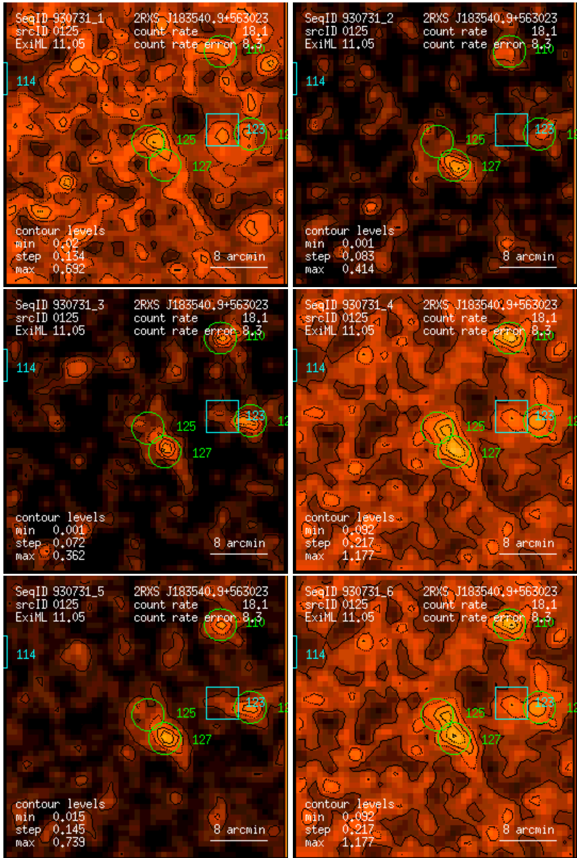
Figure 125: RASS 930731: detection 0125: band rate images, Gaussian filter: (1) PSPC channels 11 – 41, (2) 52 – 90, (3) 91 – 201, (4) 11 – 235, (5) 52 – 201, (6) 11 – 201. Broad band rates in counts/ks. Band rate contour levels in counts/ks/arcmin 2 .
