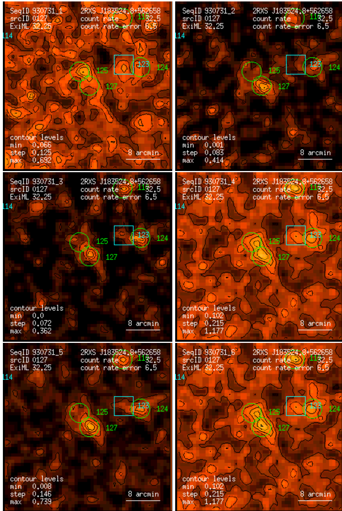
Figure 127: RASS 930731: detection 0127: band rate images, Gaussian filter: (1) PSPC channels 11 – 41, (2) 52 – 90, (3) 91 – 201, (4) 11 – 235, (5) 52 – 201, (6) 11 – 201. Broad band rates in counts/ks. Band rate contour levels in counts/ks/arcmin 2 .
