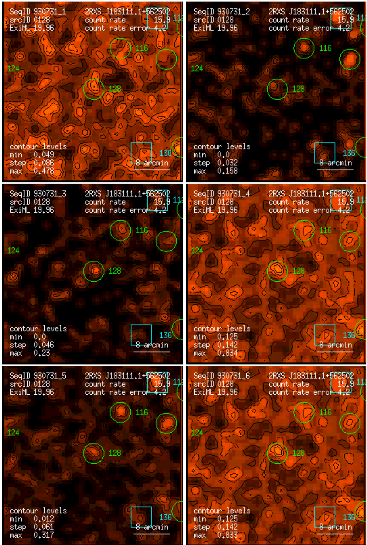
Figure 128: RASS 930731: detection 0128: band rate images, Gaussian filter: (1) PSPC channels 11 – 41, (2) 52 – 90, (3) 91 – 201, (4) 11 – 235, (5) 52 – 201, (6) 11 – 201. Broad band rates in counts/ks. Band rate contour levels in counts/ks/arcmin 2 .
