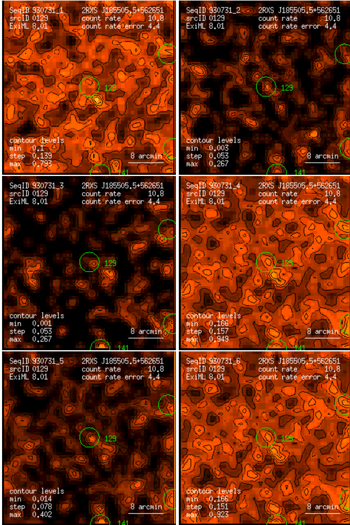
Figure 129: RASS 930731: detection 0129: band rate images, Gaussian filter: (1) PSPC channels 11 – 41, (2) 52 – 90, (3) 91 – 201, (4) 11 – 235, (5) 52 – 201, (6) 11 – 201. Broad band rates in counts/ks. Band rate contour levels in counts/ks/arcmin 2 .
