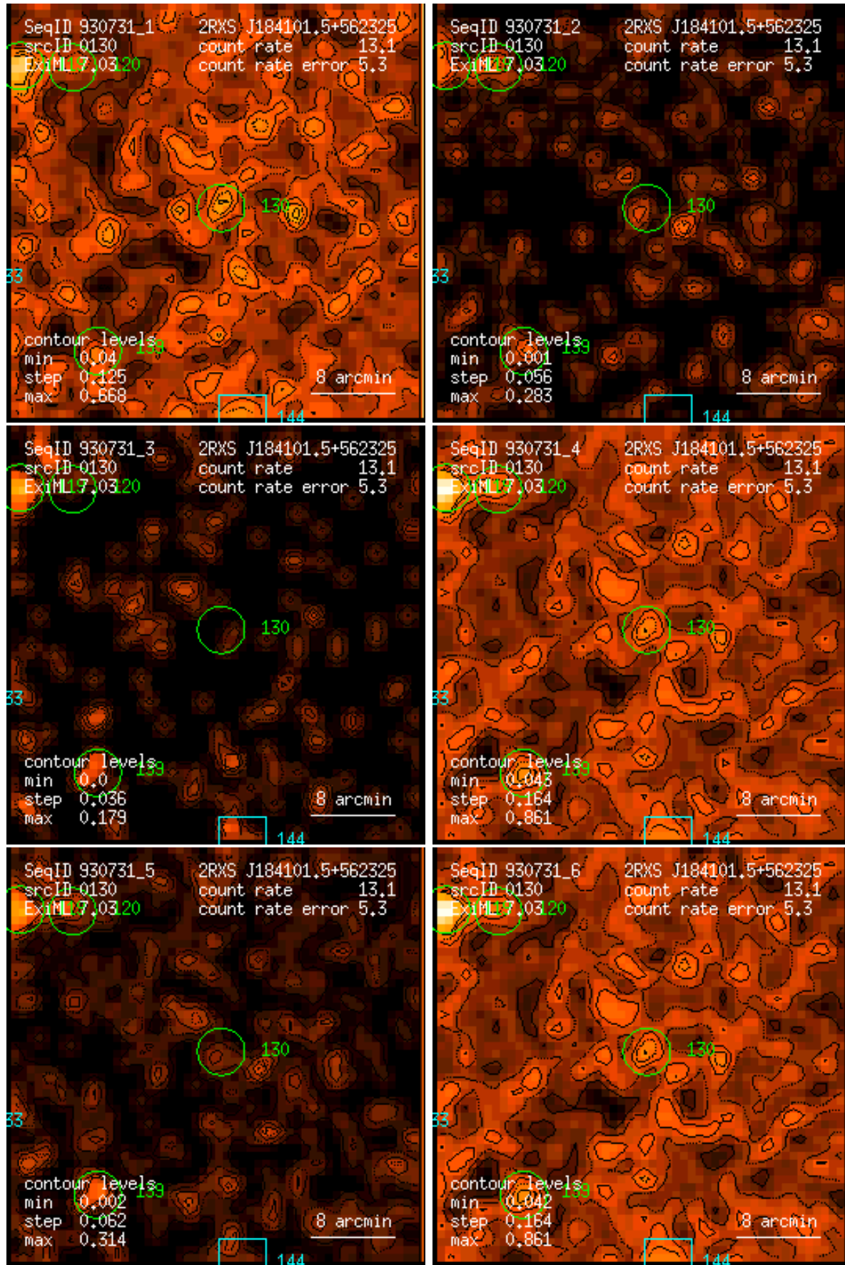
Figure 130: RASS 930731: detection 0130: band rate images, Gaussian filter: (1) PSPC channels 11 – 41, (2) 52 – 90, (3) 91 – 201, (4) 11 – 235, (5) 52 – 201, (6) 11 – 201. Broad band rates in counts/ks. Band rate contour levels in counts/ks/arcmin 2 .
