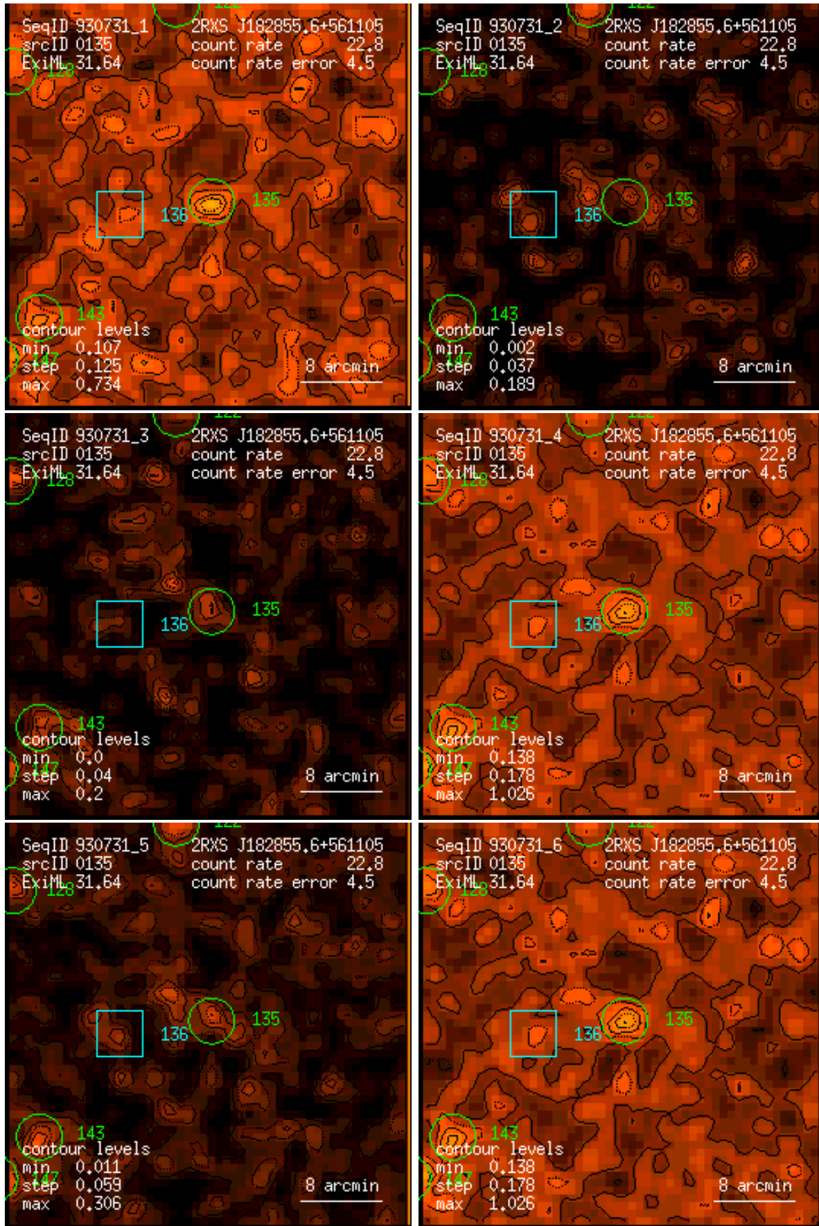
Figure 135: RASS 930731: detection 0135: band rate images, Gaussian filter: (1) PSPC channels 11 – 41, (2) 52 – 90, (3) 91 – 201, (4) 11 – 235, (5) 52 – 201, (6) 11 – 201. Broad band rates in counts/ks. Band rate contour levels in counts/ks/arcmin 2 .
