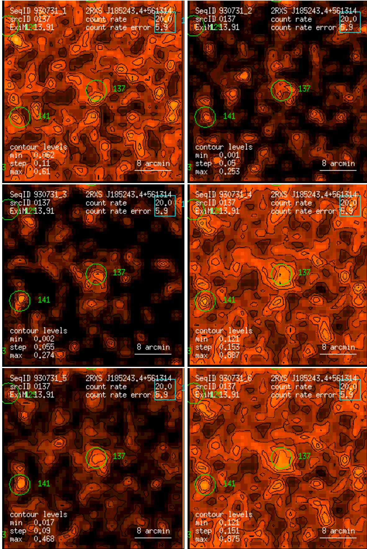
Figure 137: RASS 930731: detection 0137: band rate images, Gaussian filter: (1) PSPC channels 11 – 41, (2) 52 – 90, (3) 91 – 201, (4) 11 – 235, (5) 52 – 201, (6) 11 – 201. Broad band rates in counts/ks. Band rate contour levels in counts/ks/arcmin 2 .
