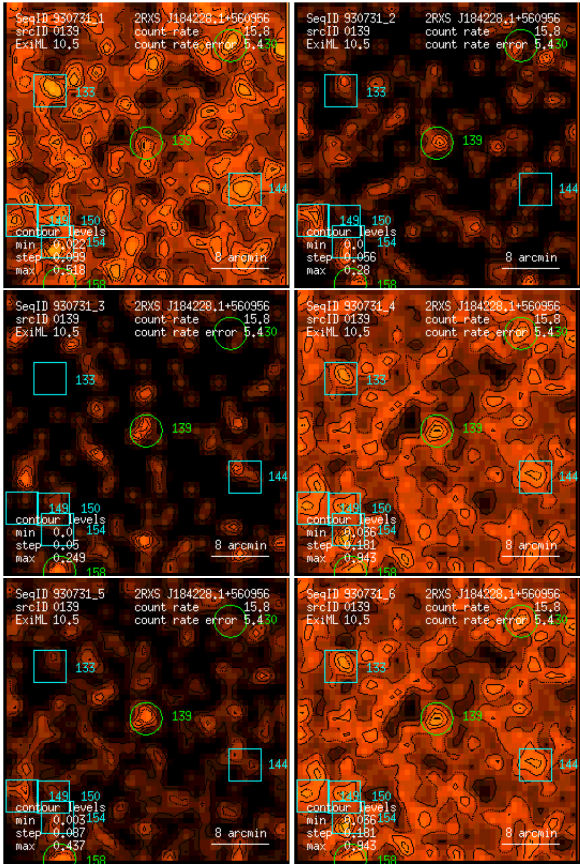
Figure 139: RASS 930731: detection 0139: band rate images, Gaussian filter: (1) PSPC channels 11 – 41, (2) 52 – 90, (3) 91 – 201, (4) 11 – 235, (5) 52 – 201, (6) 11 – 201. Broad band rates in counts/ks. Band rate contour levels in counts/ks/arcmin 2 .
