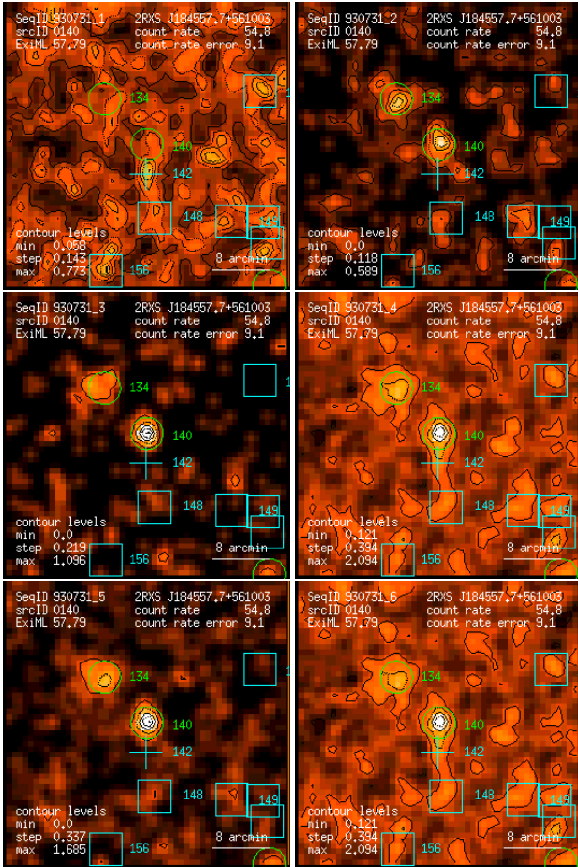
Figure 140: RASS 930731: detection 0140: band rate images, Gaussian filter: (1) PSPC channels 11 – 41, (2) 52 – 90, (3) 91 – 201, (4) 11 – 235, (5) 52 – 201, (6) 11 – 201. Broad band rates in counts/ks. Band rate contour levels in counts/ks/arcmin 2 .
