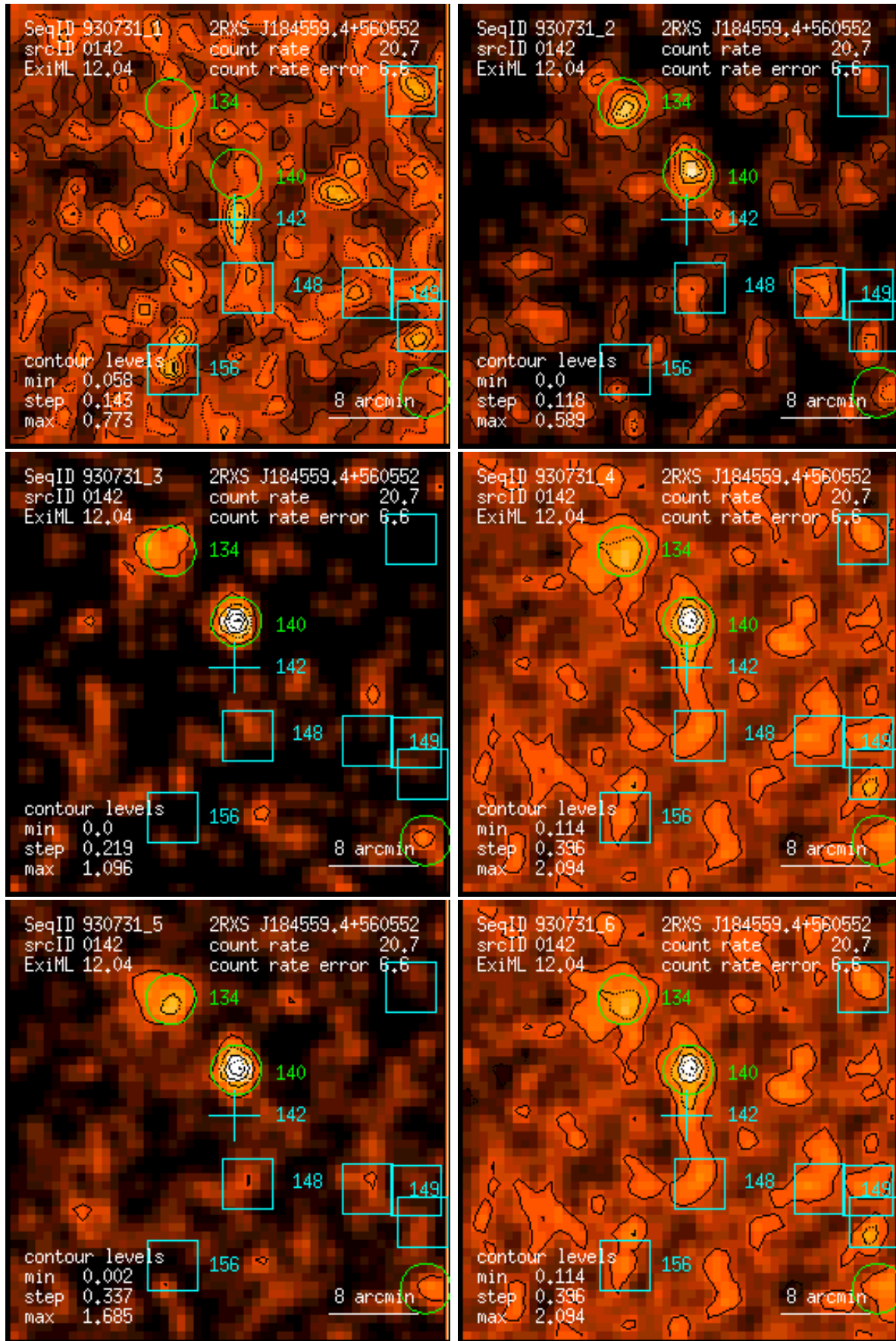
Figure 142: RASS 930731: detection 0142: band rate images, Gaussian filter: (1) PSPC channels 11 – 41, (2) 52 – 90, (3) 91 – 201, (4) 11 – 235, (5) 52 – 201, (6) 11 – 201. Broad band rates in counts/ks. Band rate contour levels in counts/ks/arcmin 2 .
