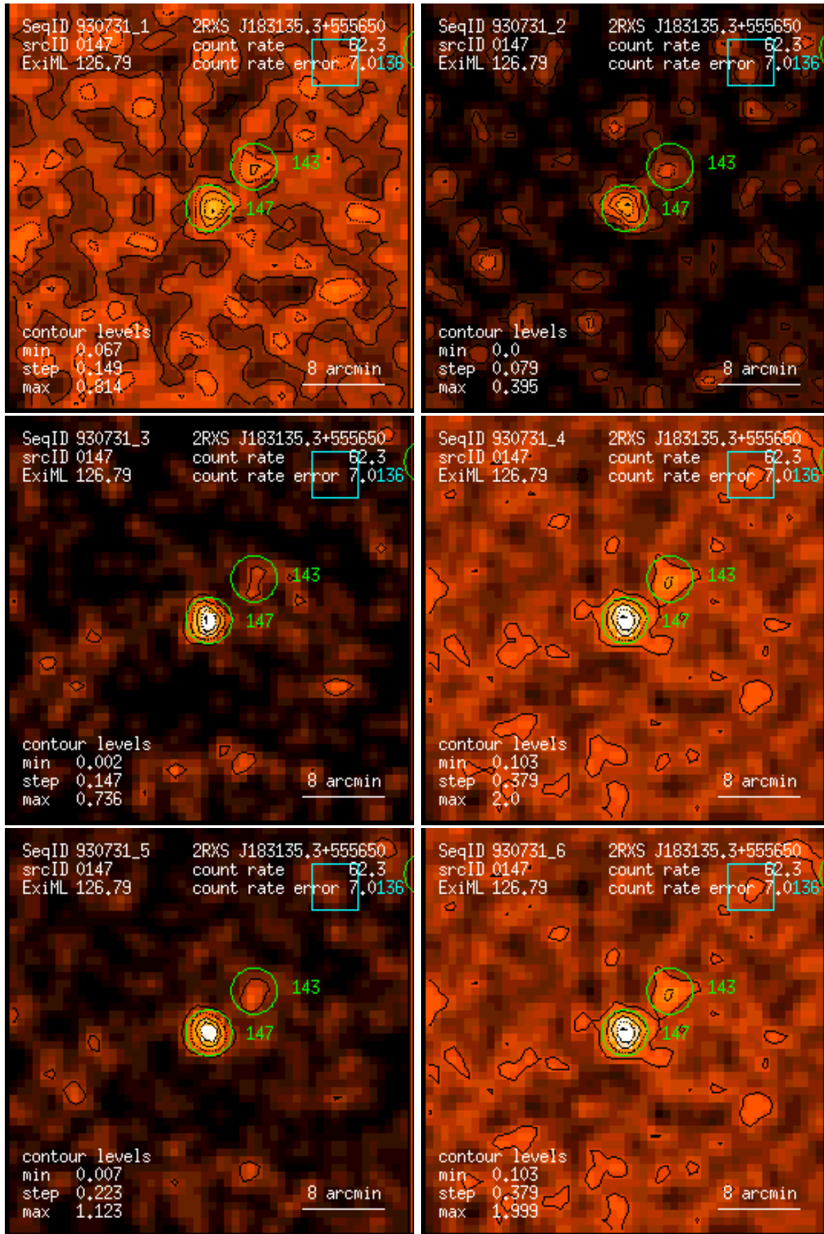
Figure 147: RASS 930731: detection 0147: band rate images, Gaussian filter: (1) PSPC channels 11 – 41, (2) 52 – 90, (3) 91 – 201, (4) 11 – 235, (5) 52 – 201, (6) 11 – 201. Broad band rates in counts/ks. Band rate contour levels in counts/ks/arcmin 2 .
