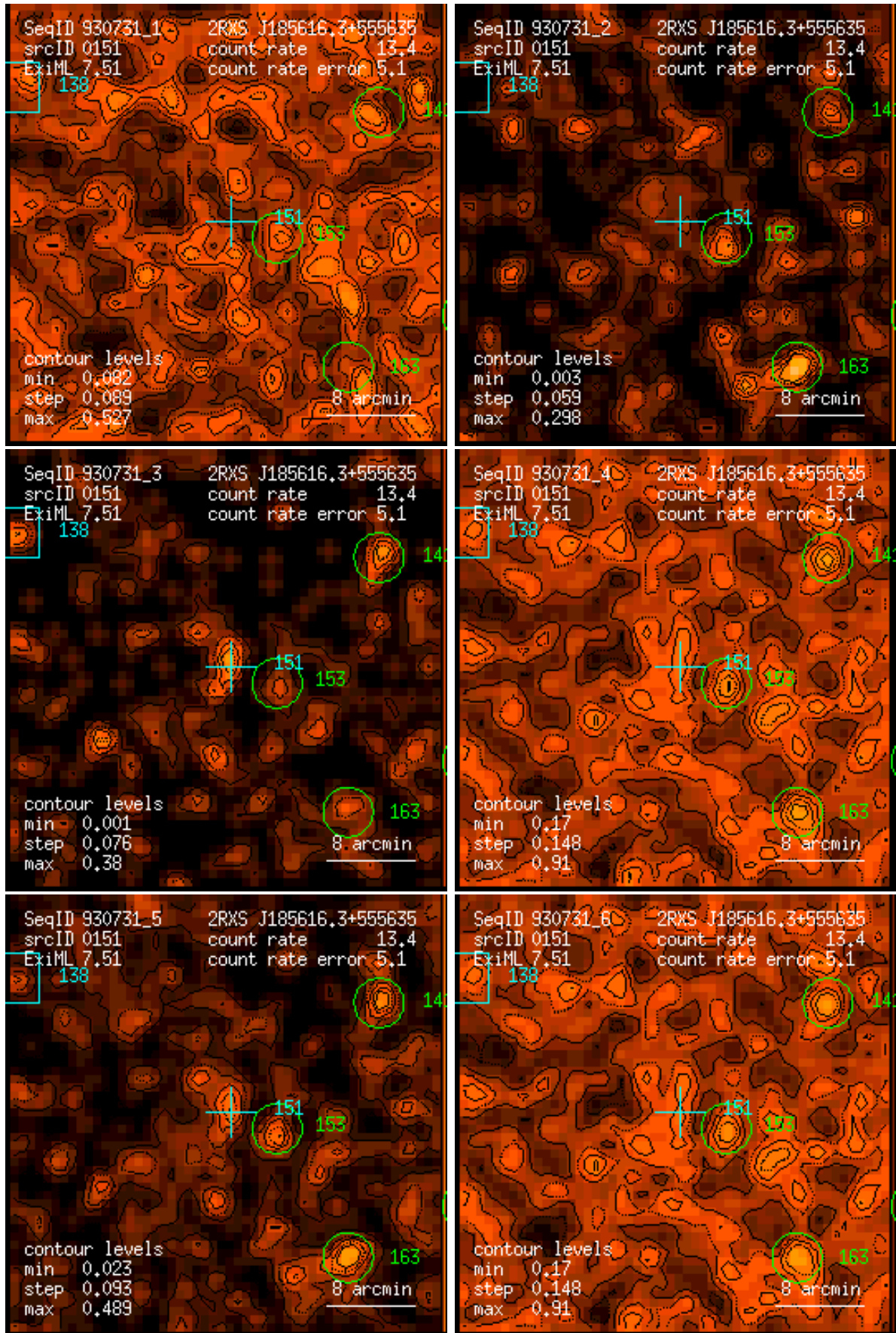
Figure 151: RASS 930731: detection 0151: band rate images, Gaussian filter: (1) PSPC channels 11 – 41, (2) 52 – 90, (3) 91 – 201, (4) 11 – 235, (5) 52 – 201, (6) 11 – 201. Broad band rates in counts/ks. Band rate contour levels in counts/ks/arcmin 2 .
