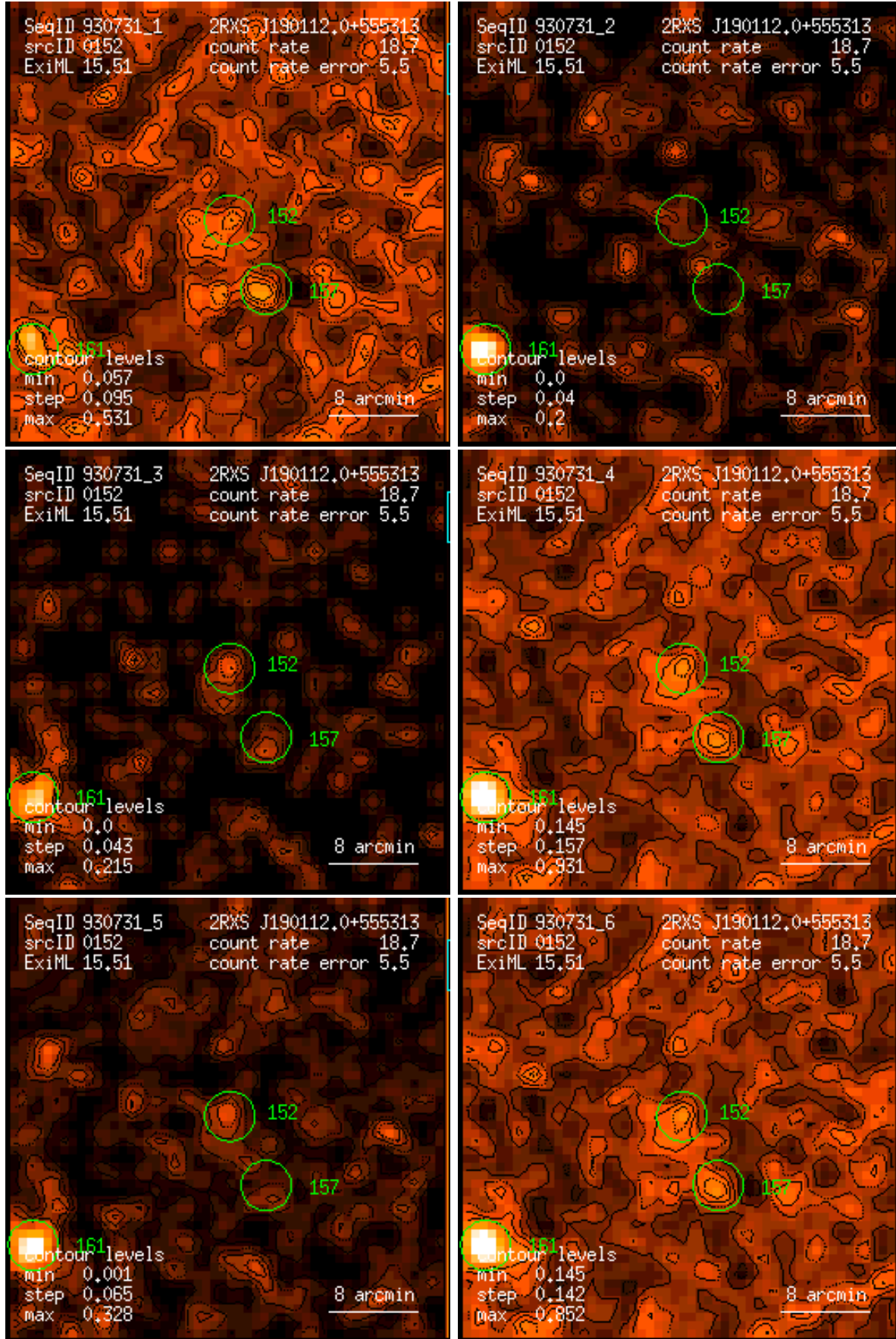
Figure 152: RASS 930731: detection 0152: band rate images, Gaussian filter: (1) PSPC channels 11 – 41, (2) 52 – 90, (3) 91 – 201, (4) 11 – 235, (5) 52 – 201, (6) 11 – 201. Broad band rates in counts/ks. Band rate contour levels in counts/ks/arcmin 2 .
