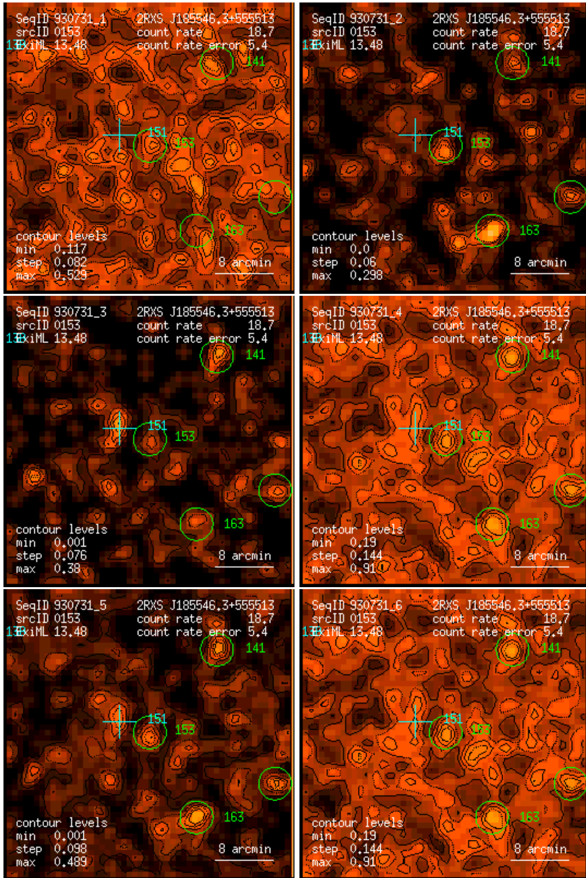
Figure 153: RASS 930731: detection 0153: band rate images, Gaussian filter: (1) PSPC channels 11 – 41, (2) 52 – 90, (3) 91 – 201, (4) 11 – 235, (5) 52 – 201, (6) 11 – 201. Broad band rates in counts/ks. Band rate contour levels in counts/ks/arcmin 2 .
