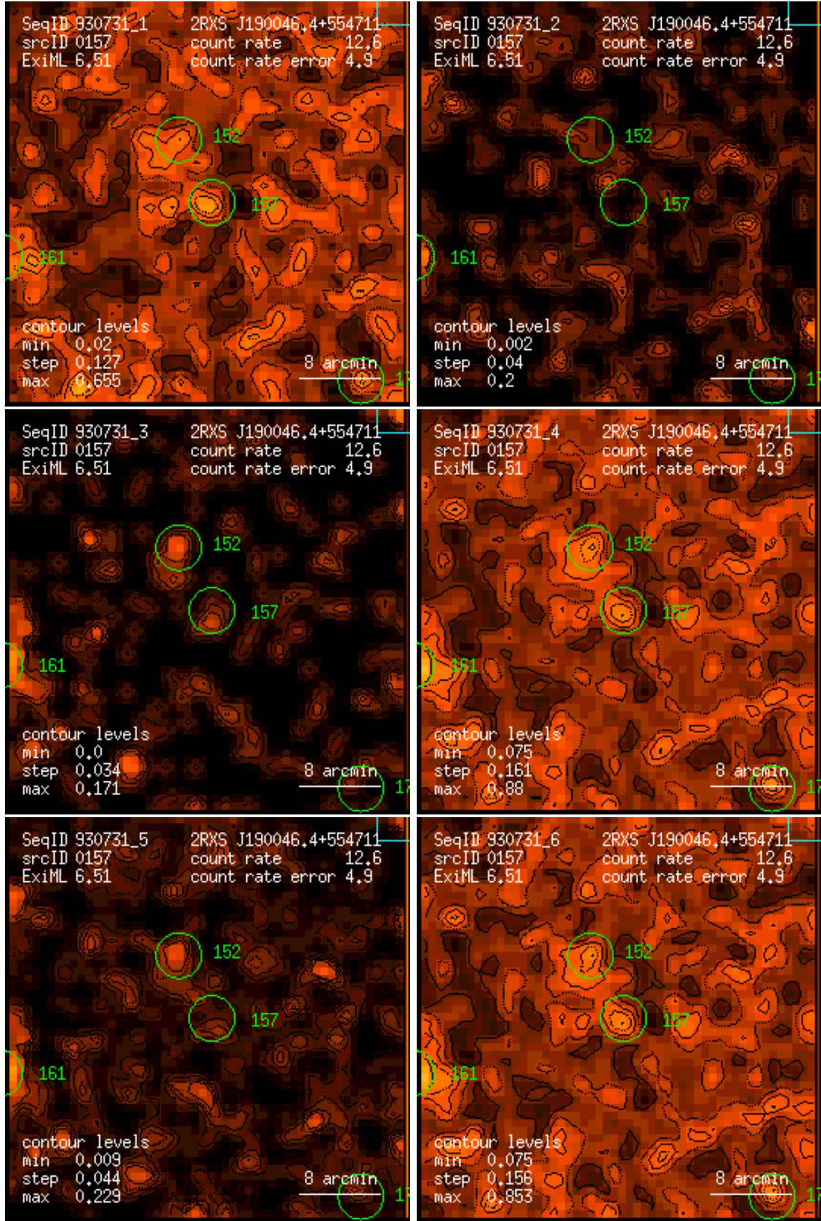
Figure 157: RASS 930731: detection 0157: band rate images, Gaussian filter: (1) PSPC channels 11 – 41, (2) 52 – 90, (3) 91 – 201, (4) 11 – 235, (5) 52 – 201, (6) 11 – 201. Broad band rates in counts/ks. Band rate contour levels in counts/ks/arcmin 2 .
