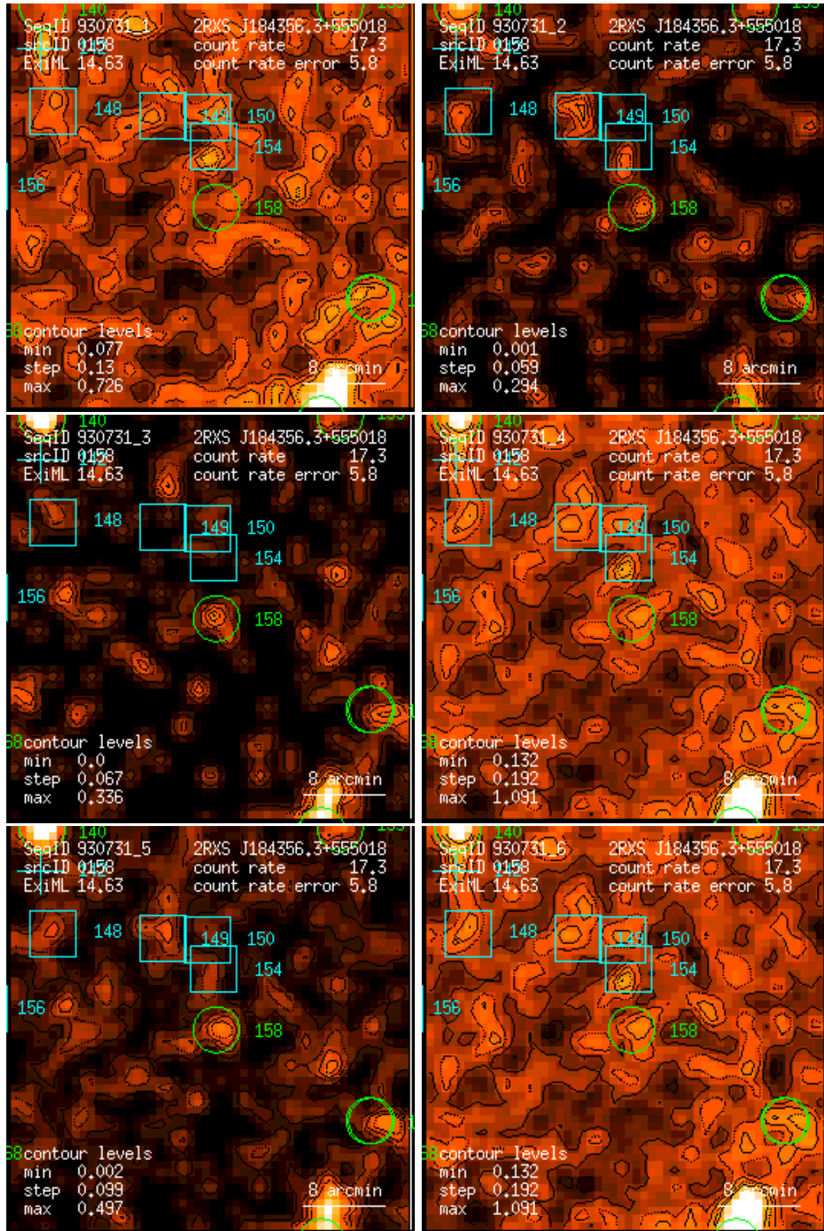
Figure 158: RASS 930731: detection 0158: band rate images, Gaussian filter: (1) PSPC channels 11 – 41, (2) 52 – 90, (3) 91 – 201, (4) 11 – 235, (5) 52 – 201, (6) 11 – 201. Broad band rates in counts/ks. Band rate contour levels in counts/ks/arcmin 2 .
